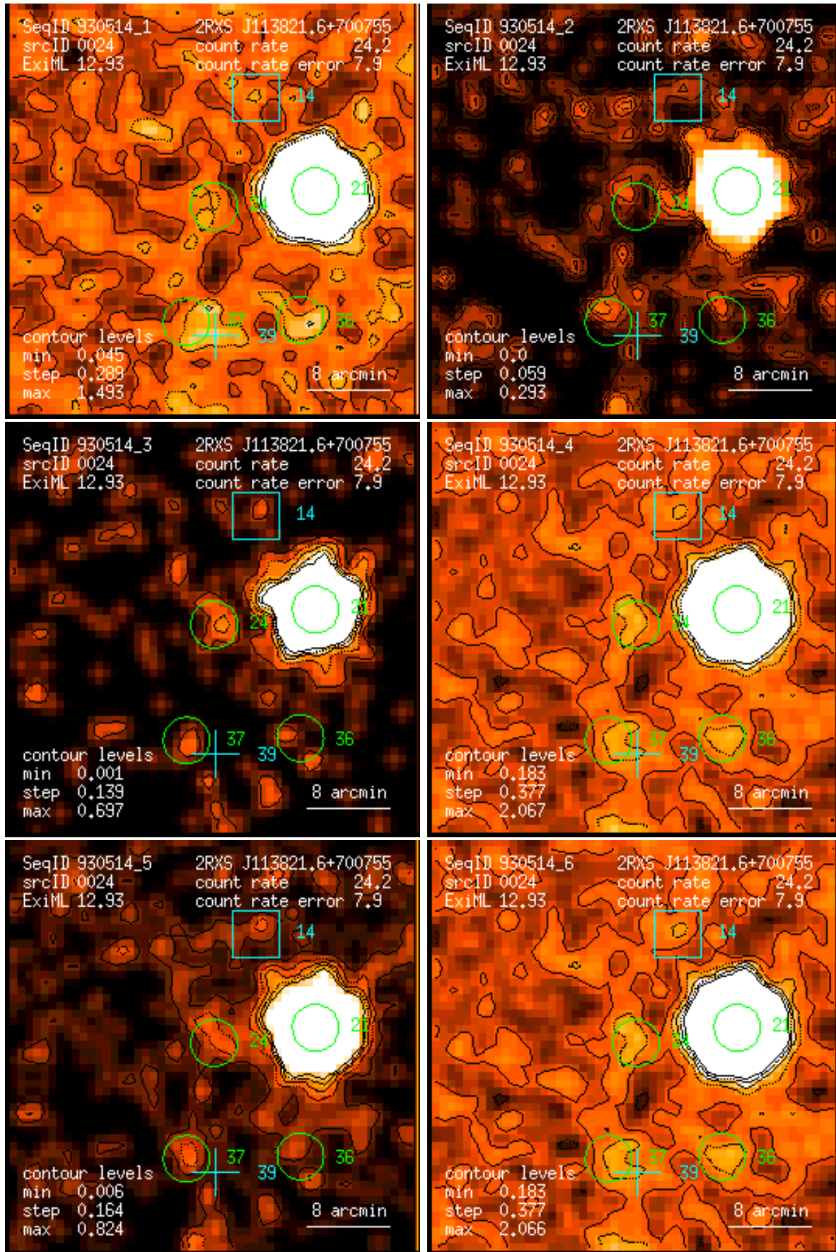
Figure 24: RASS 930514: detection 0024: band rate images, Gaussian filter: (1) PSPC channels 11 – 41, (2) 52 – 90, (3) 91 – 201, (4) 11 – 235, (5) 52 – 201, (6) 11 – 201. Broad band rates in counts/ks. Band rate contour levels in counts/ks/arcmin 2 .
