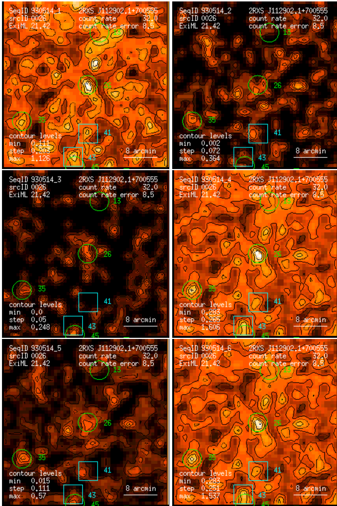
Figure 26: RASS 930514: detection 0026: band rate images, Gaussian filter: (1) PSPC channels 11 – 41, (2) 52 – 90, (3) 91 – 201, (4) 11 – 235, (5) 52 – 201, (6) 11 – 201. Broad band rates in counts/ks. Band rate contour levels in counts/ks/arcmin 2 .
