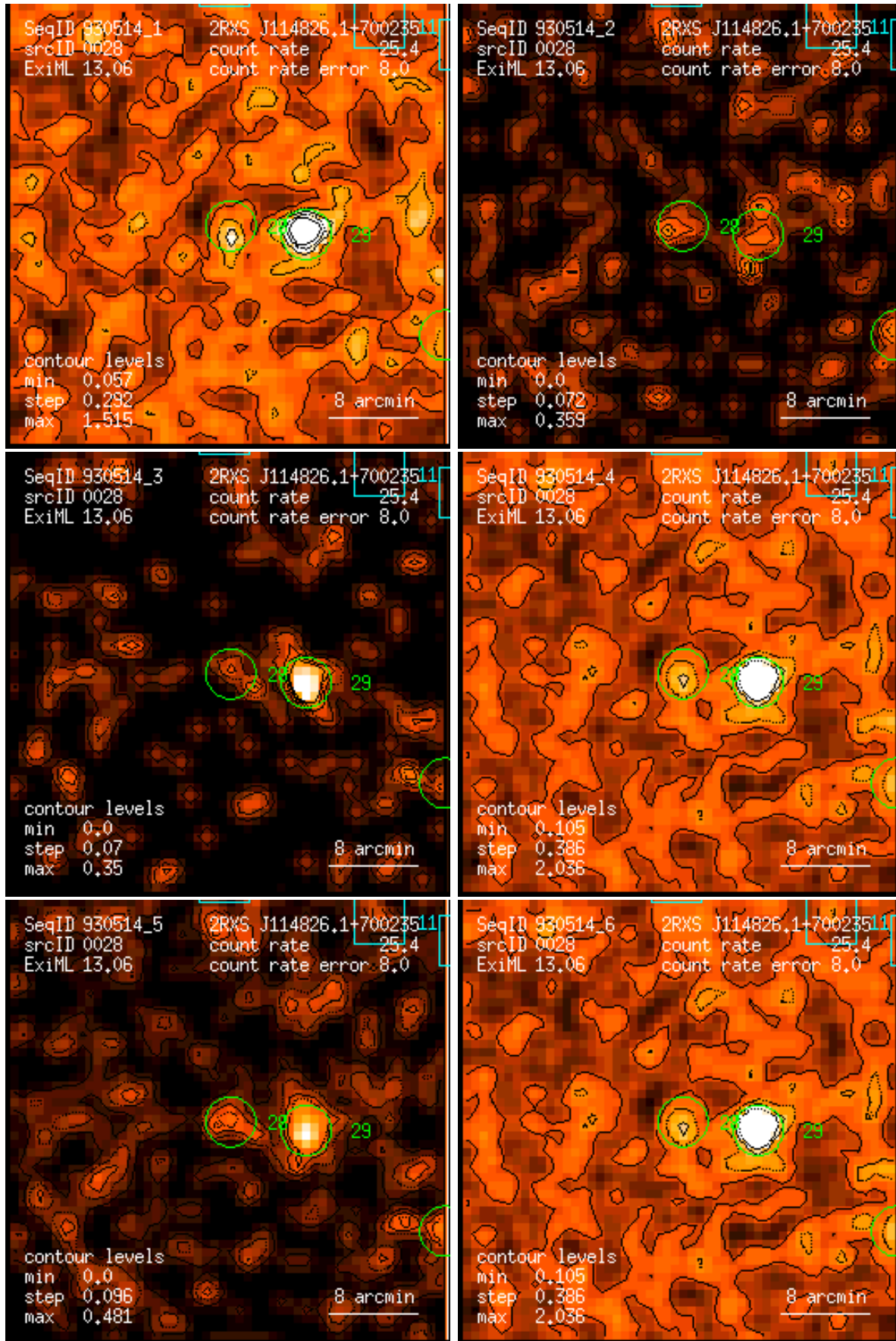
Figure 28: RASS 930514: detection 0028: band rate images, Gaussian filter: (1) PSPC channels 11 – 41, (2) 52 – 90, (3) 91 – 201, (4) 11 – 235, (5) 52 – 201, (6) 11 – 201. Broad band rates in counts/ks. Band rate contour levels in counts/ks/arcmin 2 .
