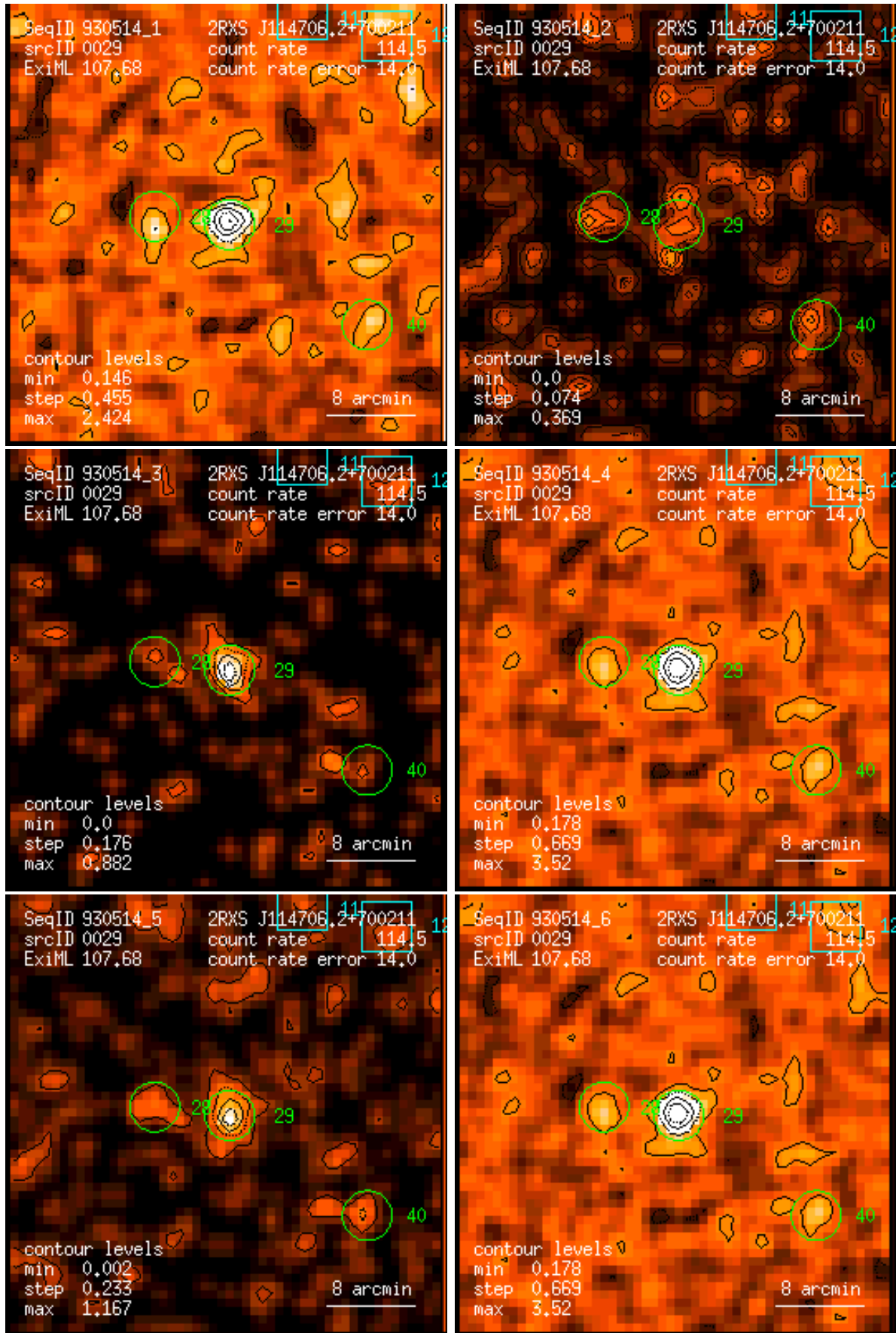
Figure 29: RASS 930514: detection 0029: band rate images, Gaussian filter: (1) PSPC channels 11 – 41, (2) 52 – 90, (3) 91 – 201, (4) 11 – 235, (5) 52 – 201, (6) 11 – 201. Broad band rates in counts/ks. Band rate contour levels in counts/ks/arcmin 2 .
