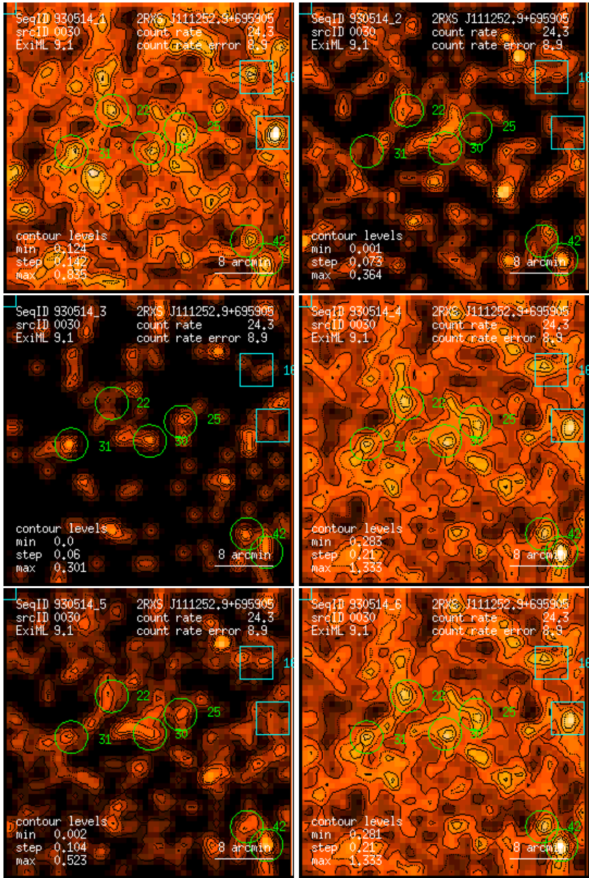
Figure 30: RASS 930514: detection 0030: band rate images, Gaussian filter: (1) PSPC channels 11 – 41, (2) 52 – 90, (3) 91 – 201, (4) 11 – 235, (5) 52 – 201, (6) 11 – 201. Broad band rates in counts/ks. Band rate contour levels in counts/ks/arcmin 2 .
