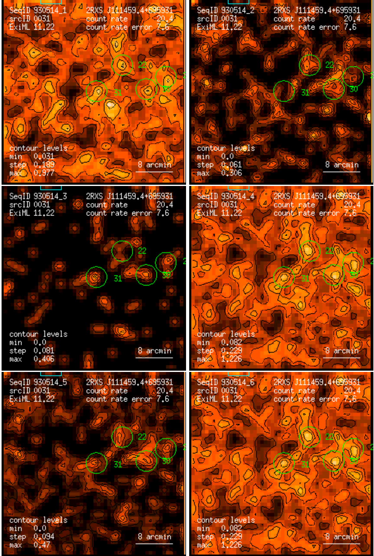
Figure 31: RASS 930514: detection 0031: band rate images, Gaussian filter: (1) PSPC channels 11 – 41, (2) 52 – 90, (3) 91 – 201, (4) 11 – 235, (5) 52 – 201, (6) 11 – 201. Broad band rates in counts/ks. Band rate contour levels in counts/ks/arcmin 2 .
