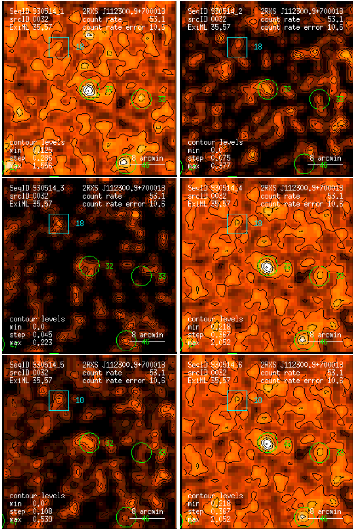
Figure 32: RASS 930514: detection 0032: band rate images, Gaussian filter: (1) PSPC channels 11 – 41, (2) 52 – 90, (3) 91 – 201, (4) 11 – 235, (5) 52 – 201, (6) 11 – 201. Broad band rates in counts/ks. Band rate contour levels in counts/ks/arcmin 2 .
