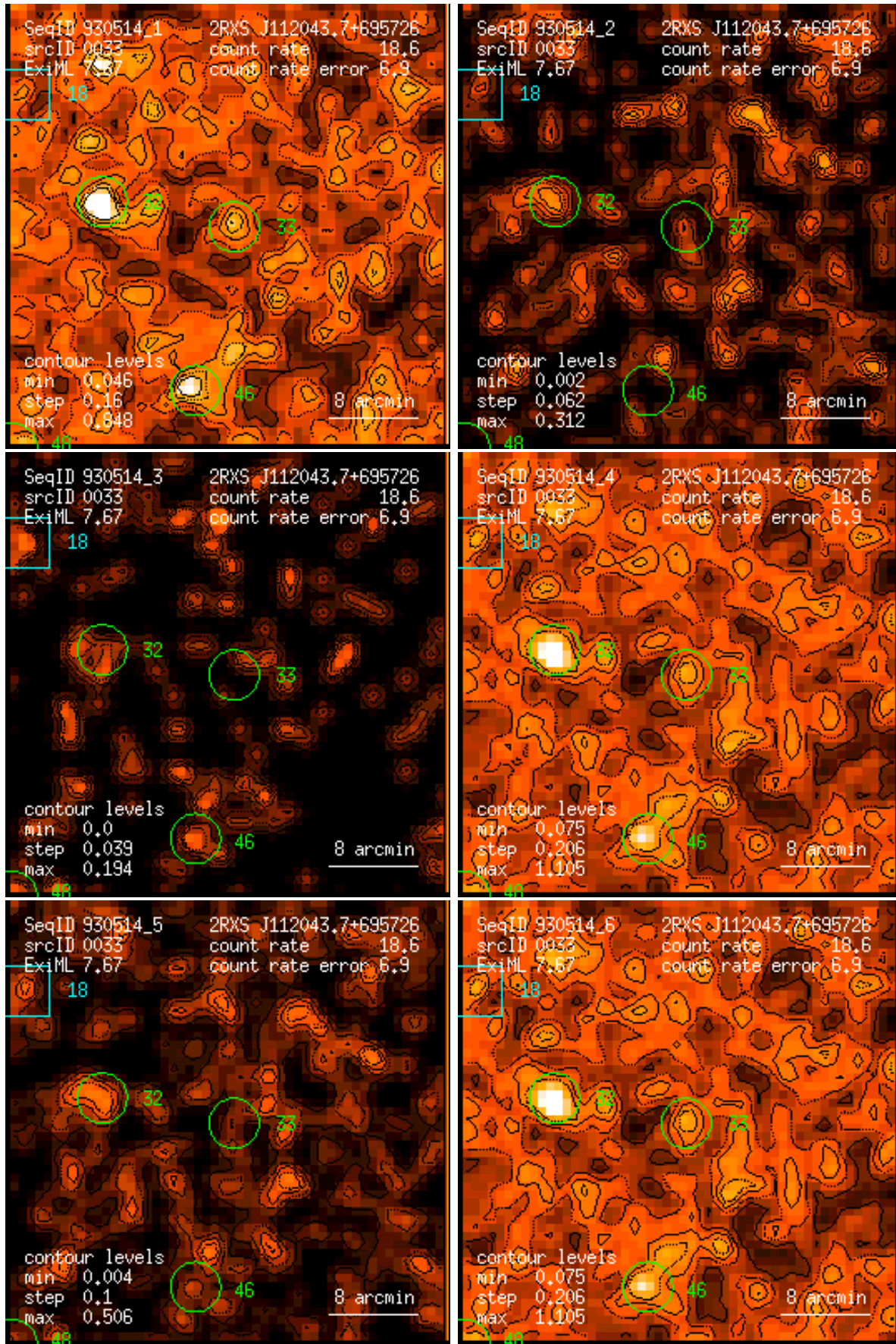
Figure 33: RASS 930514: detection 0033: band rate images, Gaussian filter: (1) PSPC channels 11 – 41, (2) 52 – 90, (3) 91 – 201, (4) 11 – 235, (5) 52 – 201, (6) 11 – 201. Broad band rates in counts/ks. Band rate contour levels in counts/ks/arcmin 2 .
