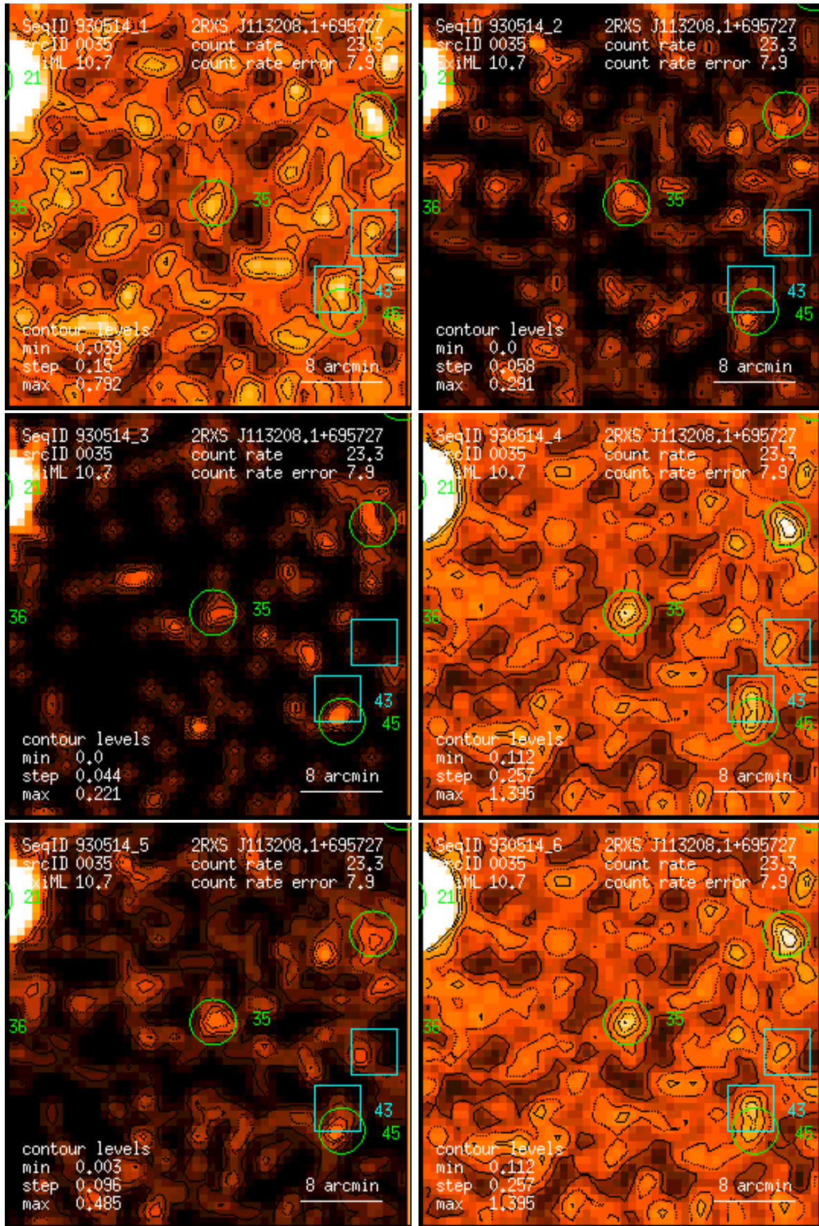
Figure 35: RASS 930514: detection 0035: band rate images, Gaussian filter: (1) PSPC channels 11 – 41, (2) 52 – 90, (3) 91 – 201, (4) 11 – 235, (5) 52 – 201, (6) 11 – 201. Broad band rates in counts/ks. Band rate contour levels in counts/ks/arcmin 2 .
