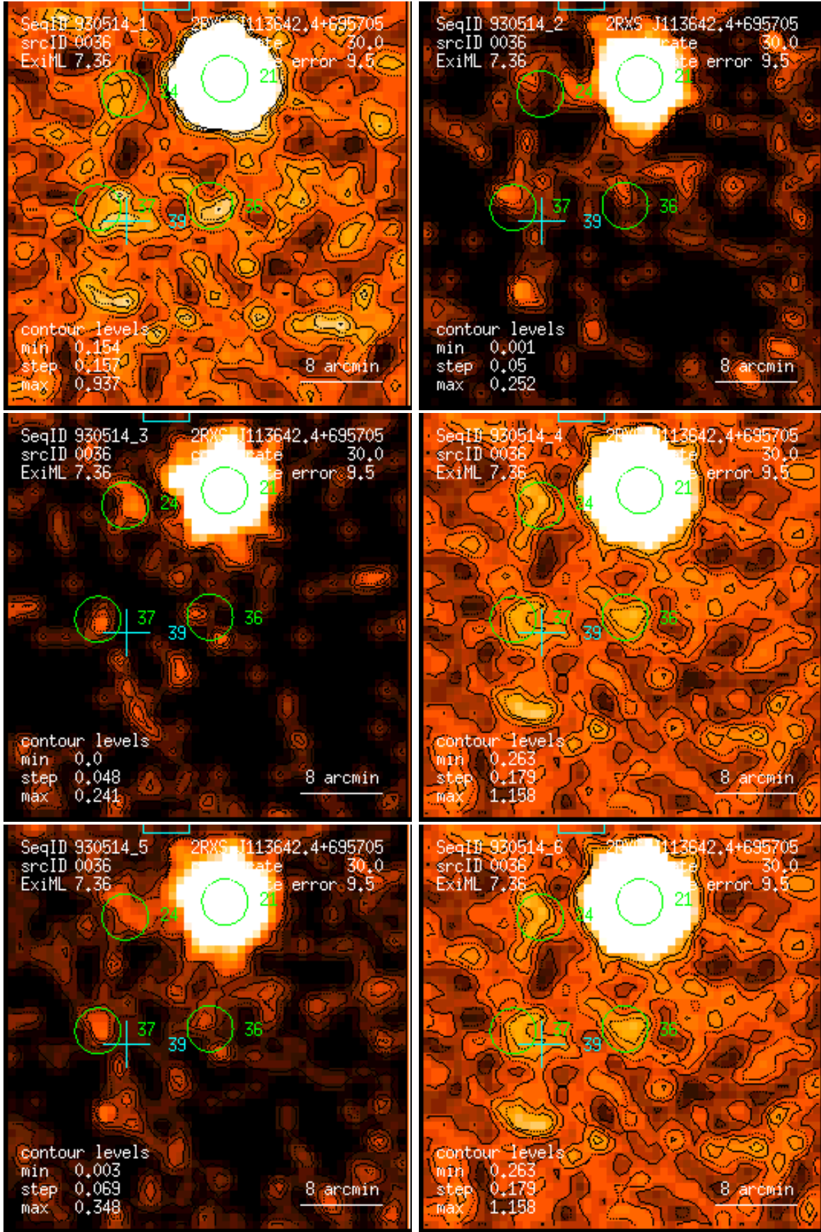
Figure 36: RASS 930514: detection 0036: band rate images, Gaussian filter: (1) PSPC channels 11 – 41, (2) 52 – 90, (3) 91 – 201, (4) 11 – 235, (5) 52 – 201, (6) 11 – 201. Broad band rates in counts/ks. Band rate contour levels in counts/ks/arcmin 2 .
