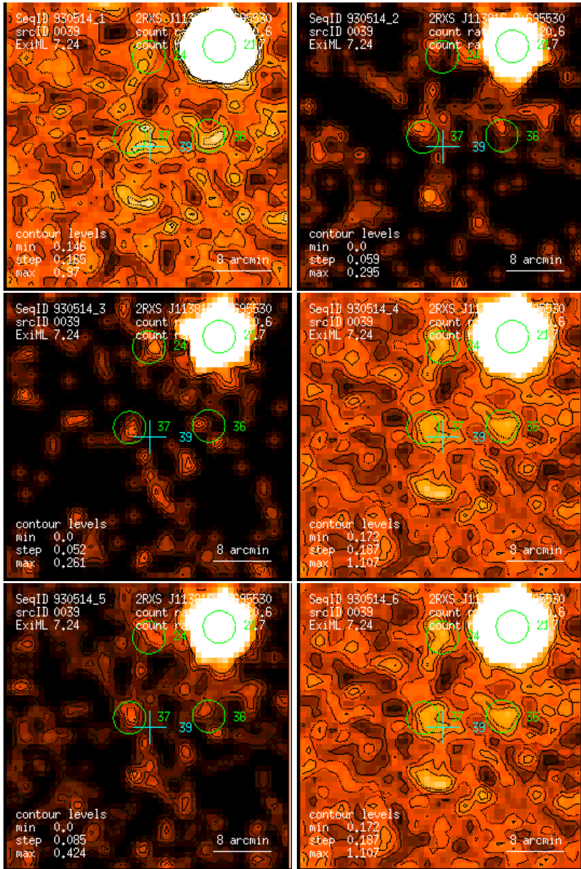
Figure 39: RASS 930514: detection 0039: band rate images, Gaussian filter: (1) PSPC channels 11 – 41, (2) 52 – 90, (3) 91 – 201, (4) 11 – 235, (5) 52 – 201, (6) 11 – 201. Broad band rates in counts/ks. Band rate contour levels in counts/ks/arcmin 2 .
