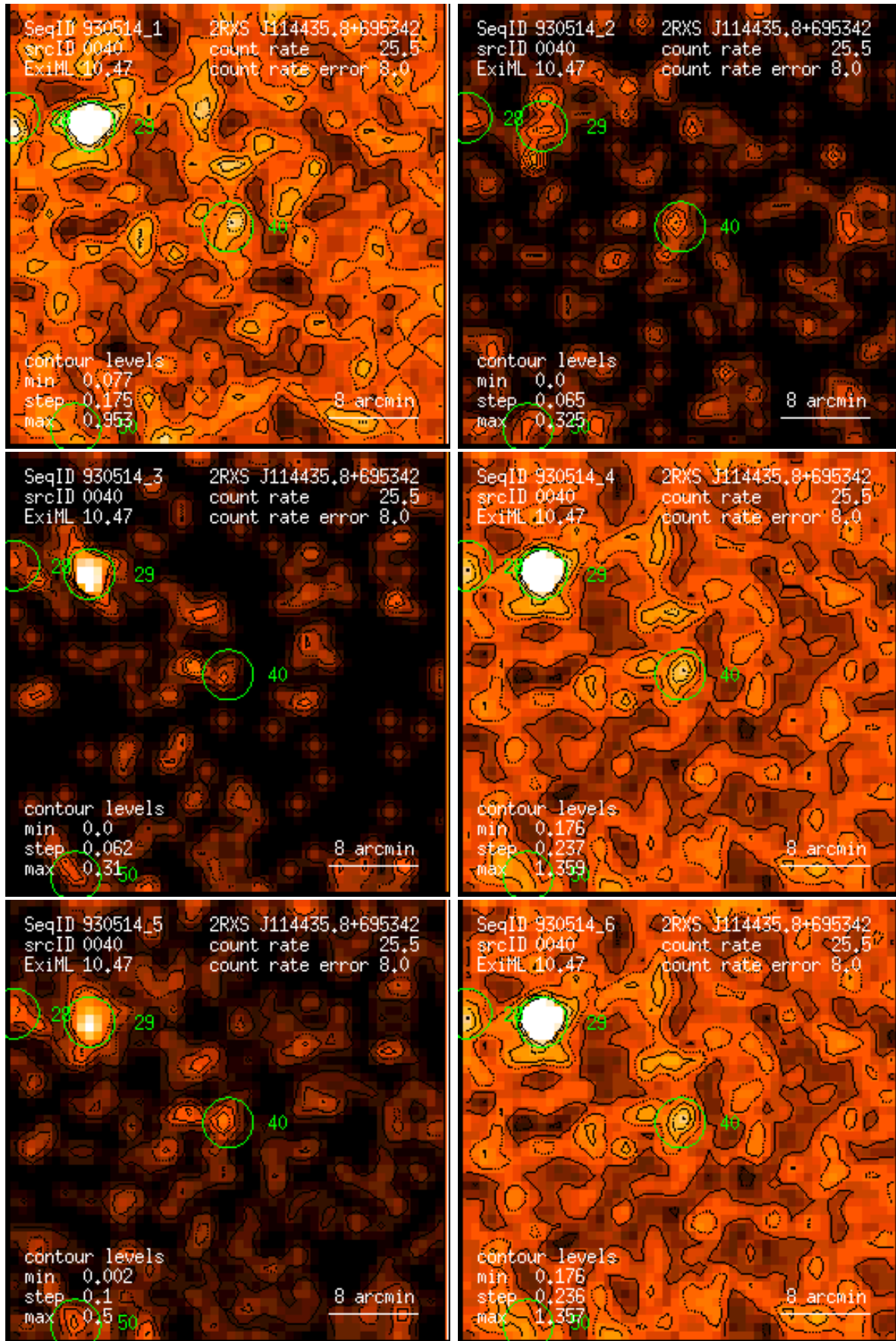
Figure 40: RASS 930514: detection 0040: band rate images, Gaussian filter: (1) PSPC channels 11 – 41, (2) 52 – 90, (3) 91 – 201, (4) 11 – 235, (5) 52 – 201, (6) 11 – 201. Broad band rates in counts/ks. Band rate contour levels in counts/ks/arcmin 2 .
