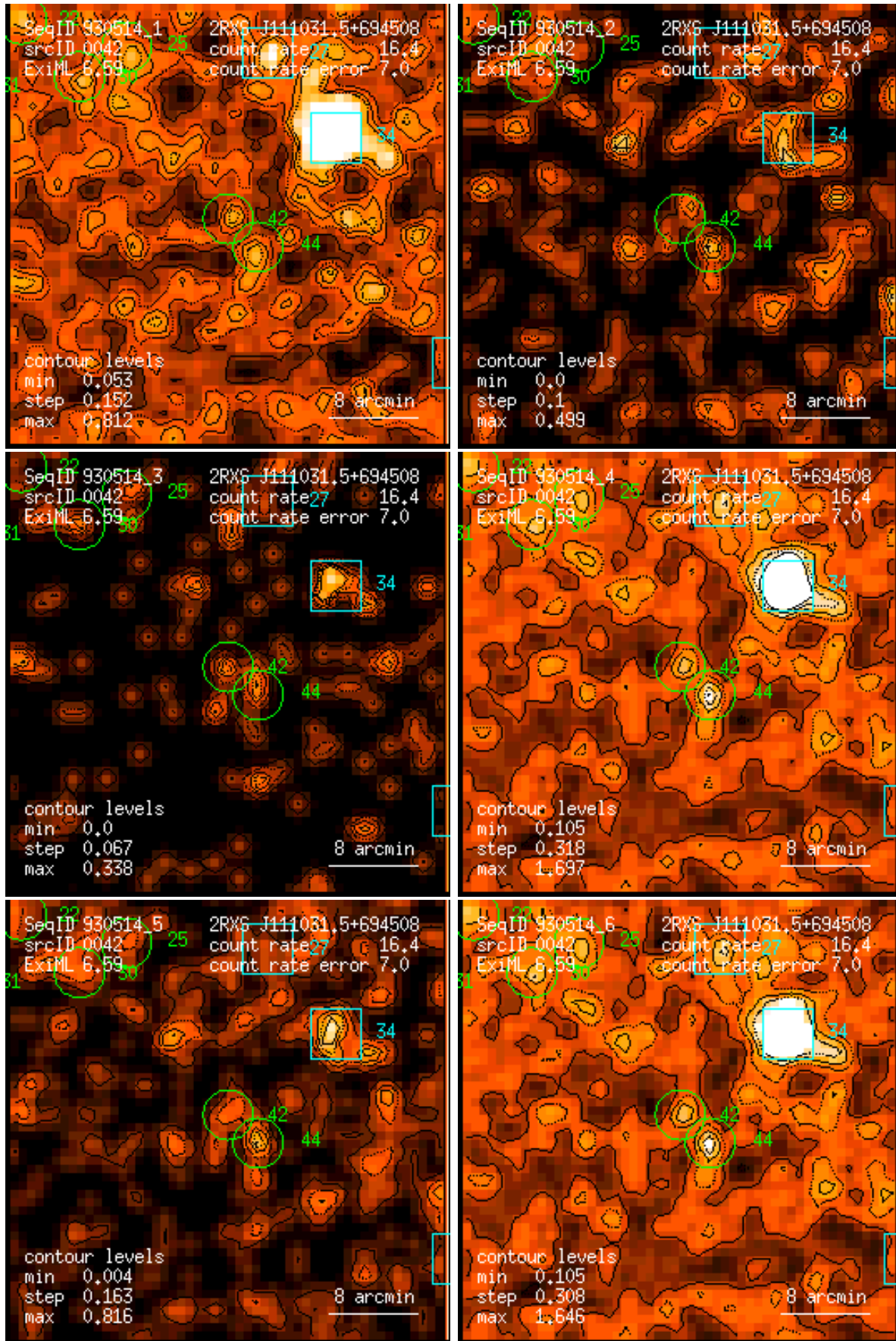
Figure 42: RASS 930514: detection 0042: band rate images, Gaussian filter: (1) PSPC channels 11 – 41, (2) 52 – 90, (3) 91 – 201, (4) 11 – 235, (5) 52 – 201, (6) 11 – 201. Broad band rates in counts/ks. Band rate contour levels in counts/ks/arcmin 2 .
