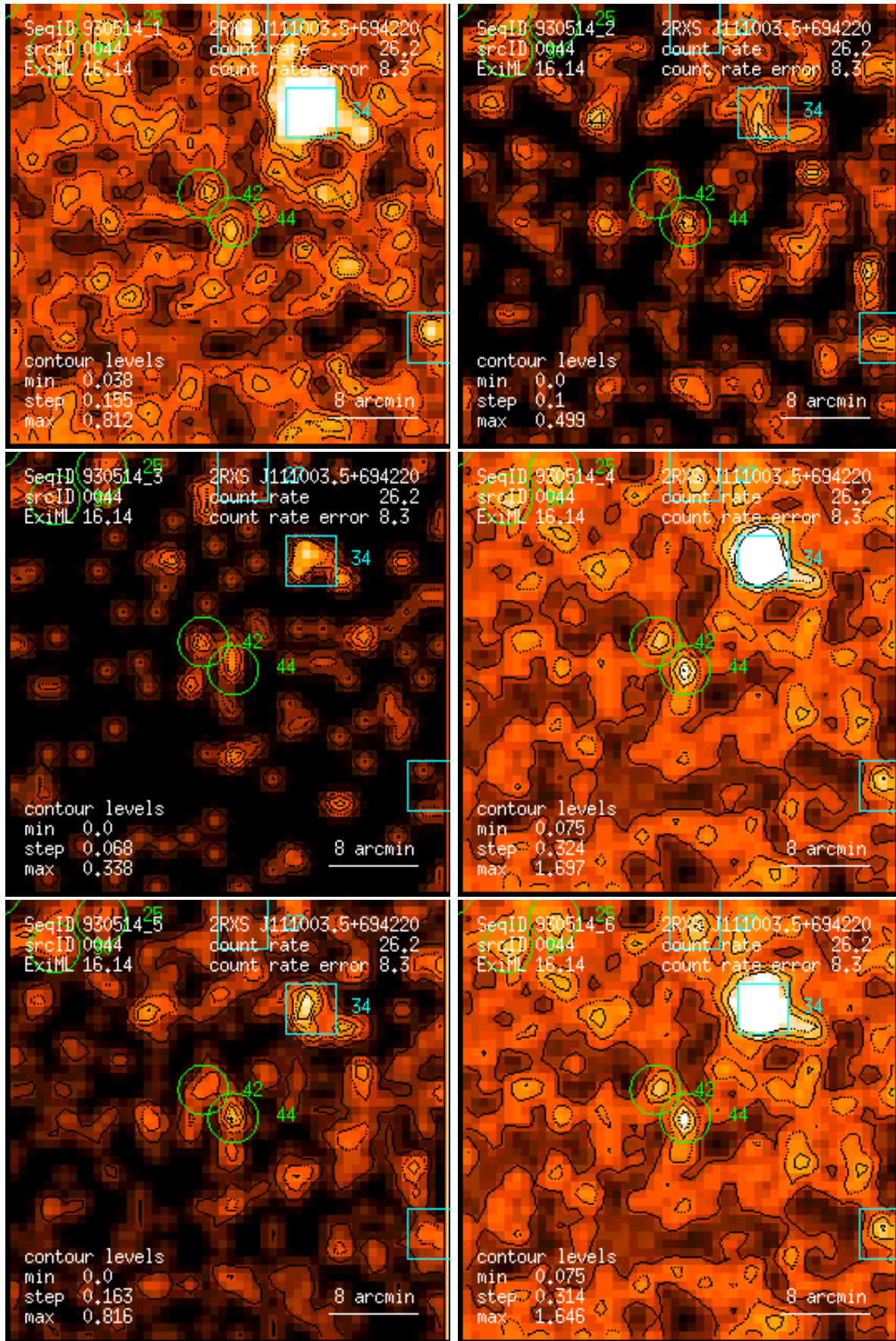
Figure 44: RASS 930514: detection 0044: band rate images, Gaussian filter: (1) PSPC channels 11 – 41, (2) 52 – 90, (3) 91 – 201, (4) 11 – 235, (5) 52 – 201, (6) 11 – 201. Broad band rates in counts/ks. Band rate contour levels in counts/ks/arcmin 2 .
