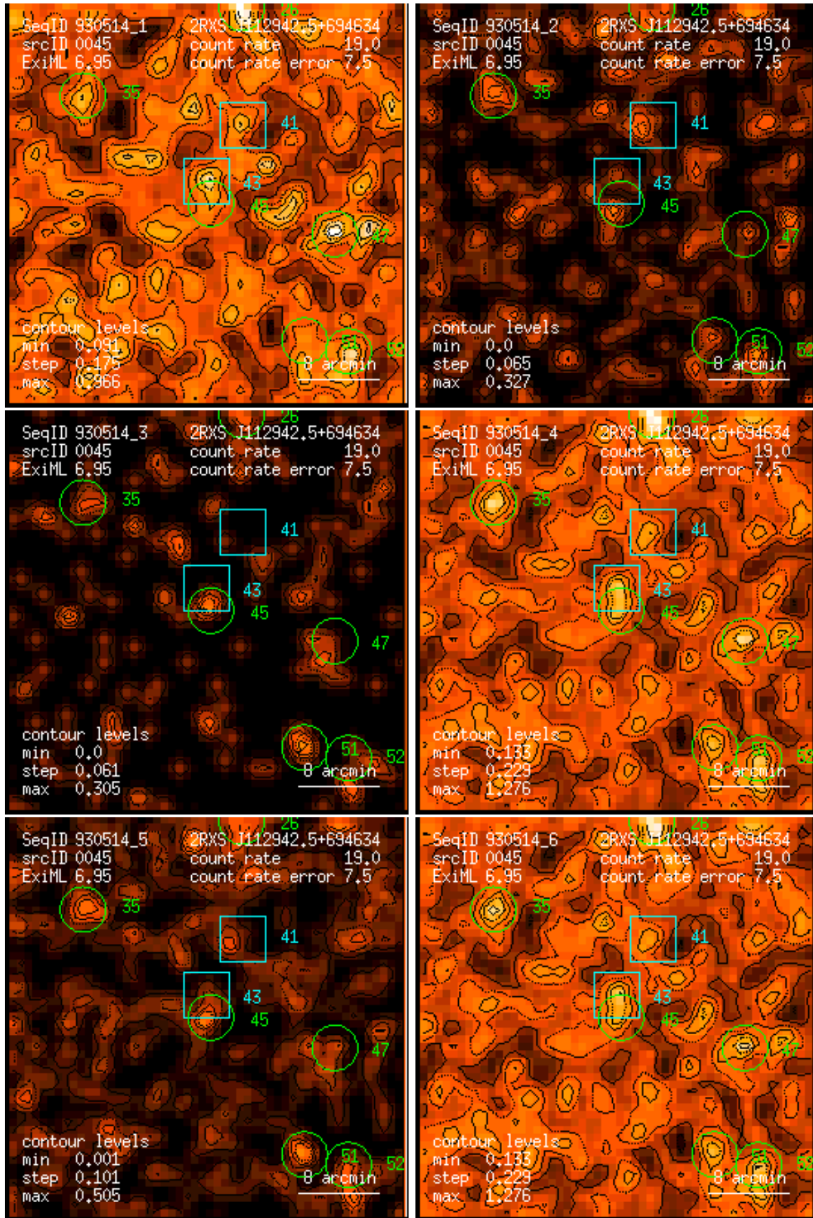
Figure 45: RASS 930514: detection 0045: band rate images, Gaussian filter: (1) PSPC channels 11 – 41, (2) 52 – 90, (3) 91 – 201, (4) 11 – 235, (5) 52 – 201, (6) 11 – 201. Broad band rates in counts/ks. Band rate contour levels in counts/ks/arcmin 2 .
