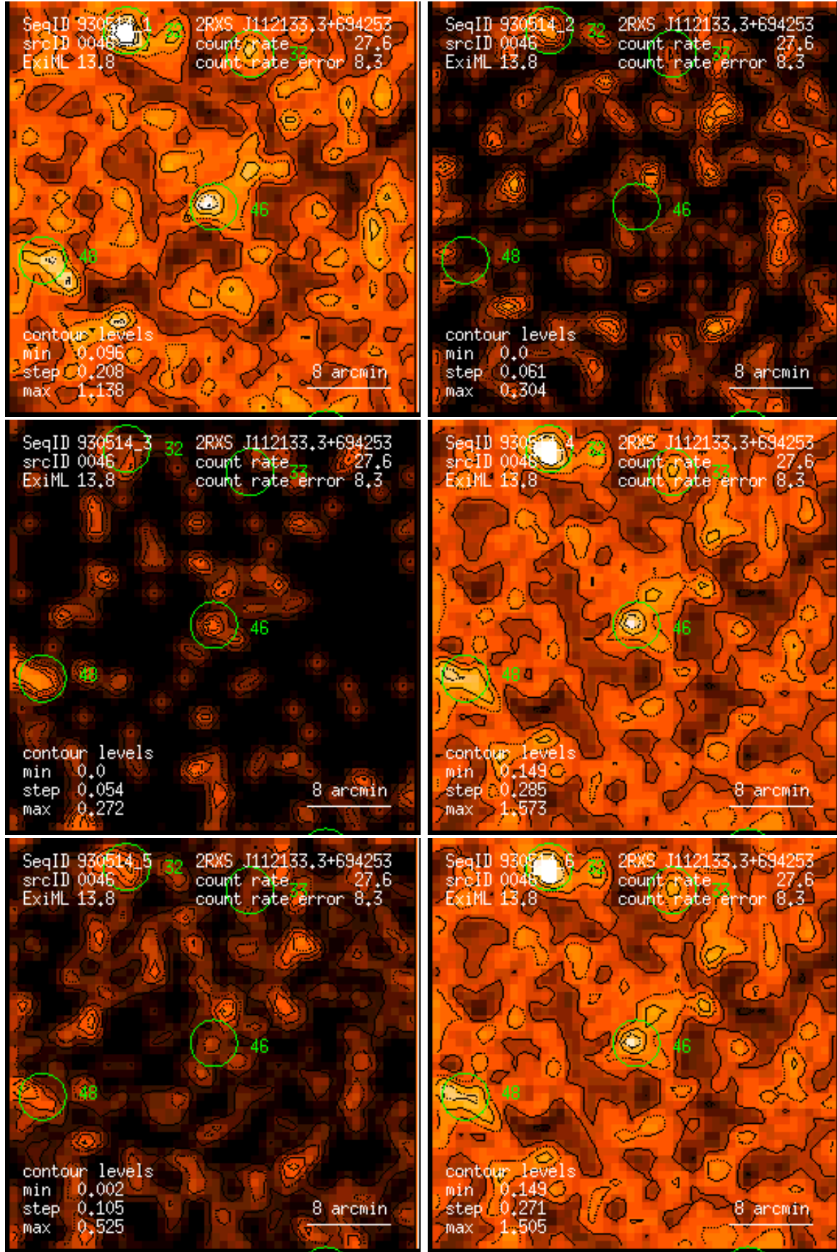
Figure 46: RASS 930514: detection 0046: band rate images, Gaussian filter: (1) PSPC channels 11 – 41, (2) 52 – 90, (3) 91 – 201, (4) 11 – 235, (5) 52 – 201, (6) 11 – 201. Broad band rates in counts/ks. Band rate contour levels in counts/ks/arcmin 2 .
