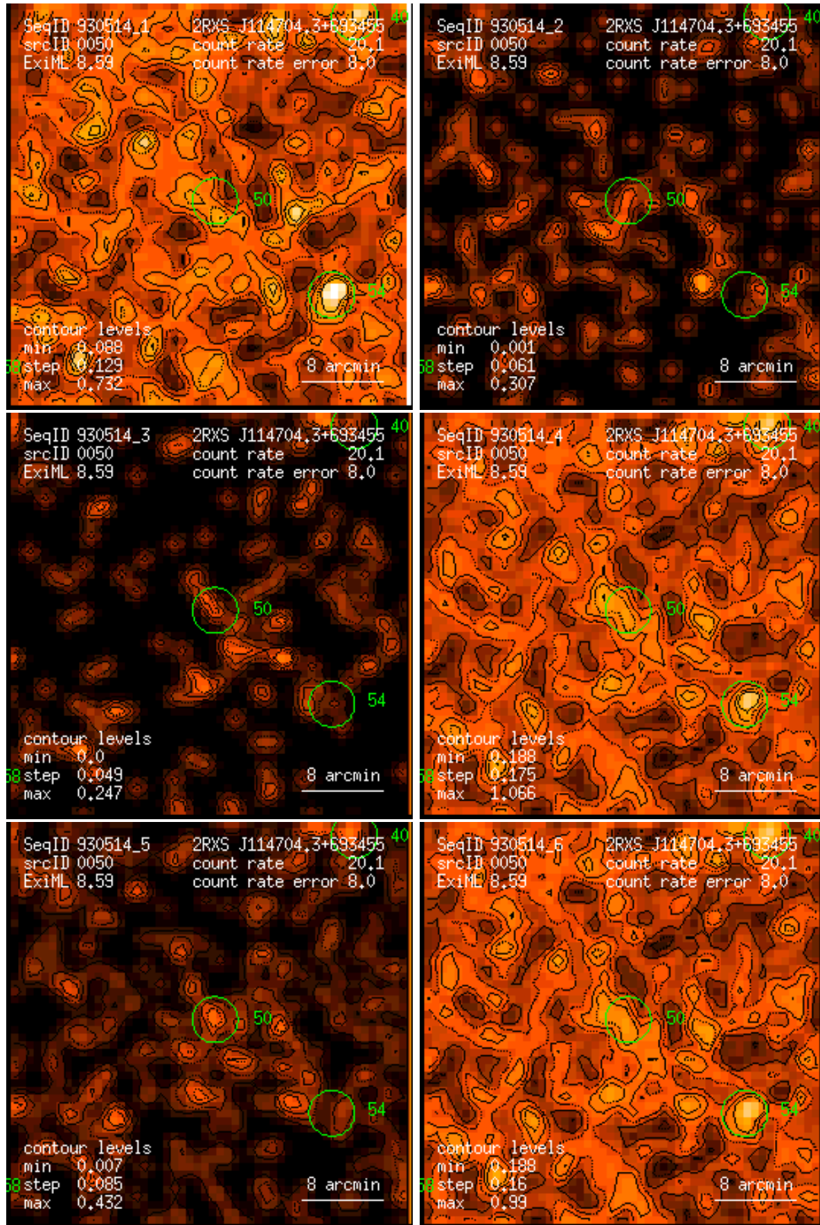
Figure 50: RASS 930514: detection 0050: band rate images, Gaussian filter: (1) PSPC channels 11 – 41, (2) 52 – 90, (3) 91 – 201, (4) 11 – 235, (5) 52 – 201, (6) 11 – 201. Broad band rates in counts/ks. Band rate contour levels in counts/ks/arcmin 2 .
