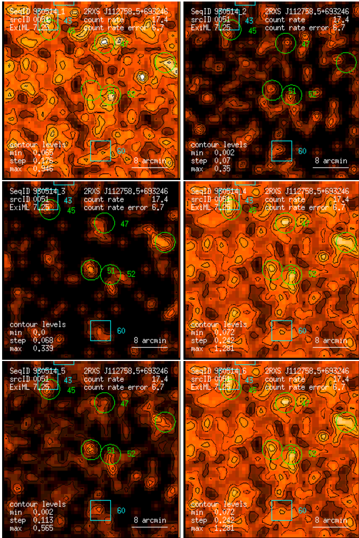
Figure 51: RASS 930514: detection 0051: band rate images, Gaussian filter: (1) PSPC channels 11 – 41, (2) 52 – 90, (3) 91 – 201, (4) 11 – 235, (5) 52 – 201, (6) 11 – 201. Broad band rates in counts/ks. Band rate contour levels in counts/ks/arcmin 2 .
