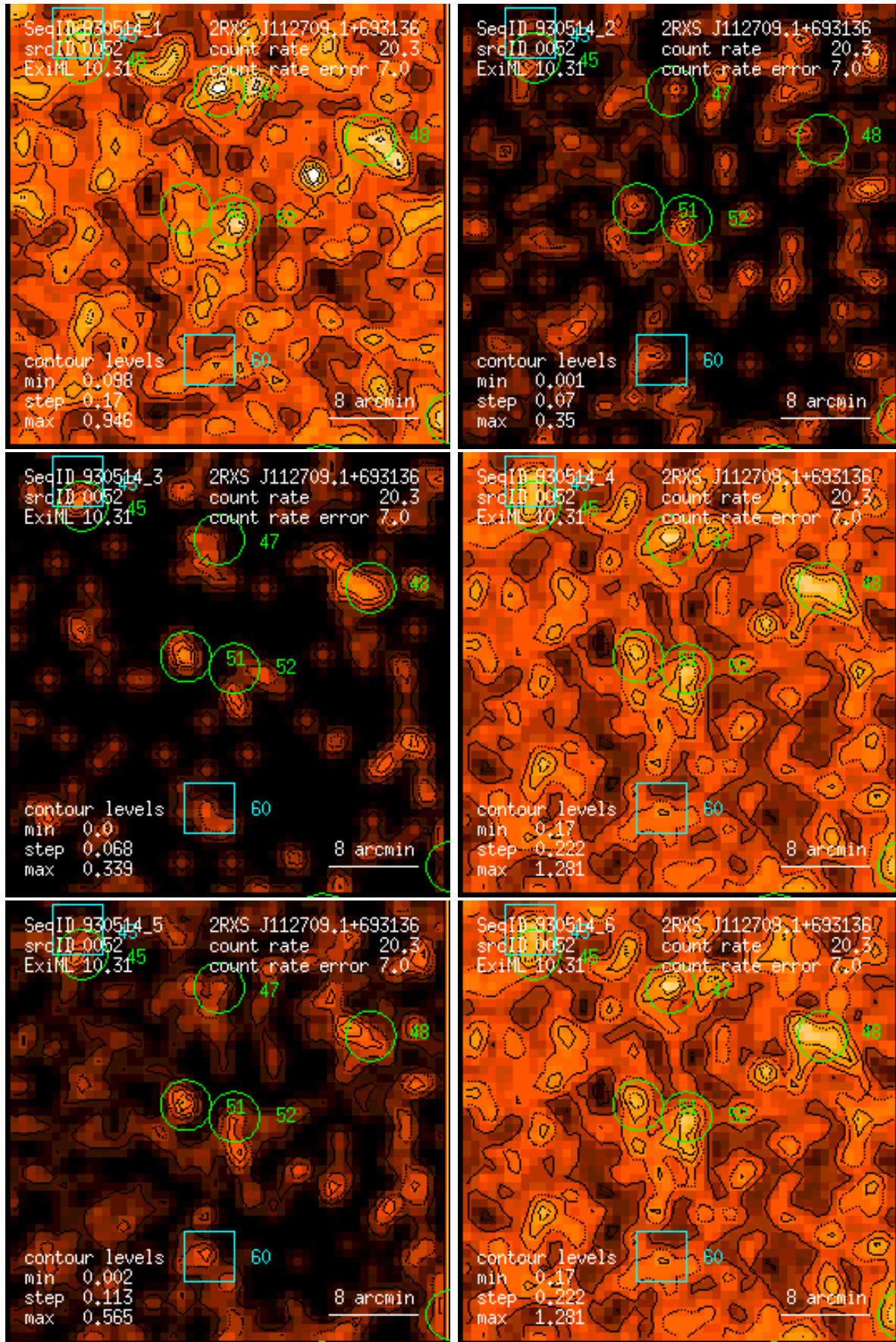
Figure 52: RASS 930514: detection 0052: band rate images, Gaussian filter: (1) PSPC channels 11 – 41, (2) 52 – 90, (3) 91 – 201, (4) 11 – 235, (5) 52 – 201, (6) 11 – 201. Broad band rates in counts/ks. Band rate contour levels in counts/ks/arcmin 2 .
