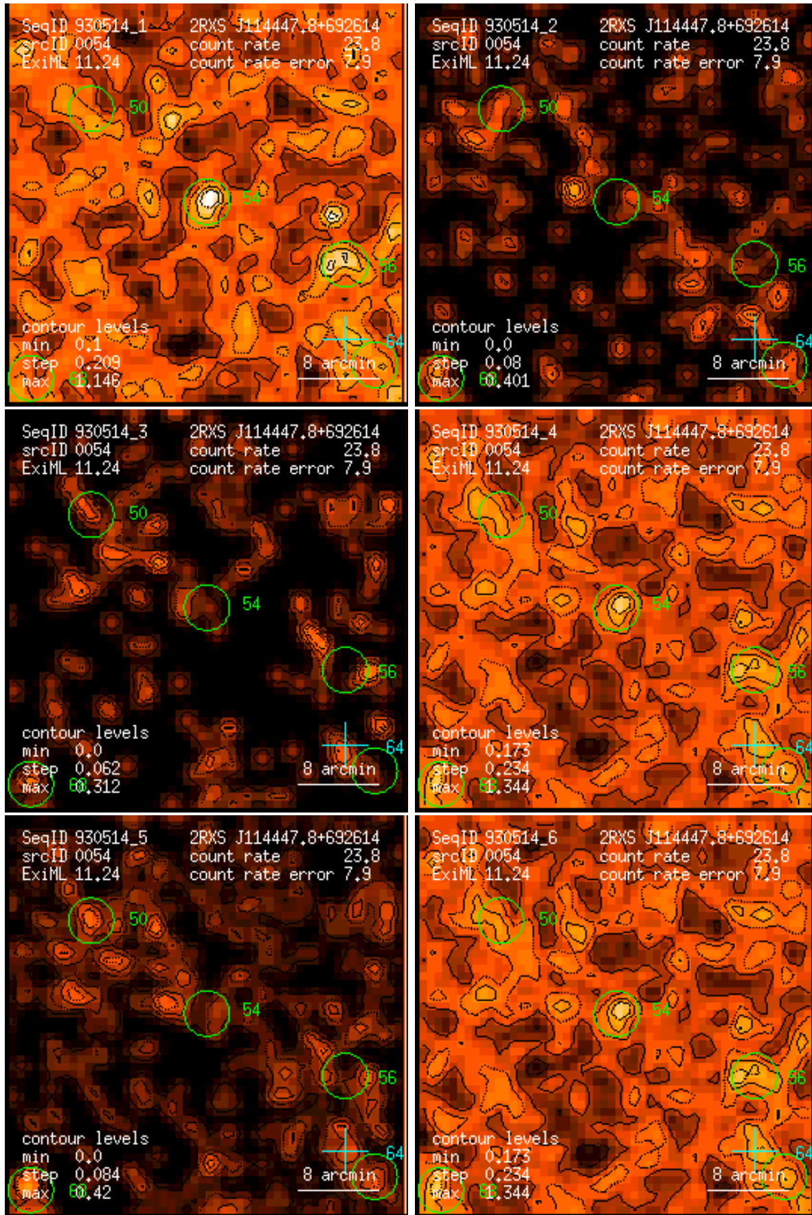
Figure 54: RASS 930514: detection 0054: band rate images, Gaussian filter: (1) PSPC channels 11 – 41, (2) 52 – 90, (3) 91 – 201, (4) 11 – 235, (5) 52 – 201, (6) 11 – 201. Broad band rates in counts/ks. Band rate contour levels in counts/ks/arcmin 2 .
