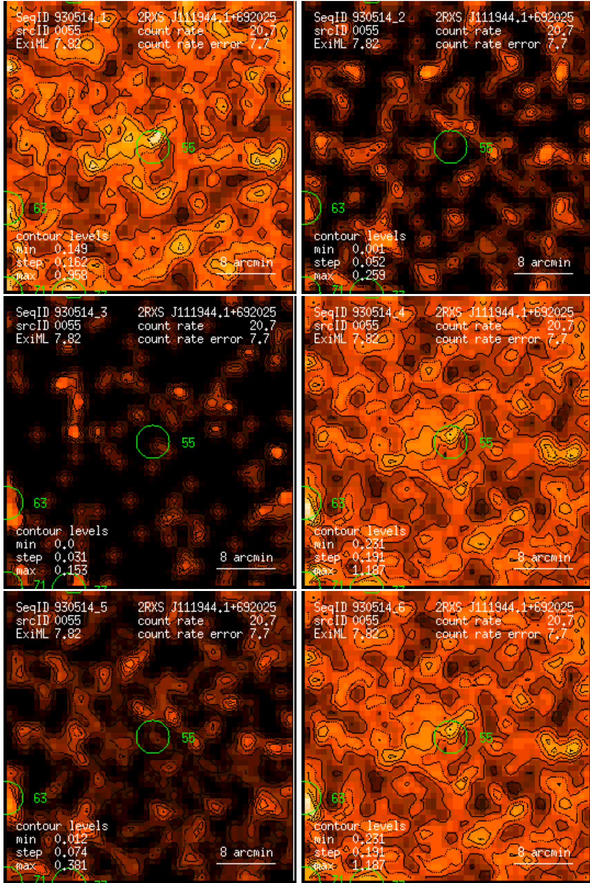
Figure 55: RASS 930514: detection 0055: band rate images, Gaussian filter: (1) PSPC channels 11 – 41, (2) 52 – 90, (3) 91 – 201, (4) 11 – 235, (5) 52 – 201, (6) 11 – 201. Broad band rates in counts/ks. Band rate contour levels in counts/ks/arcmin 2 .
