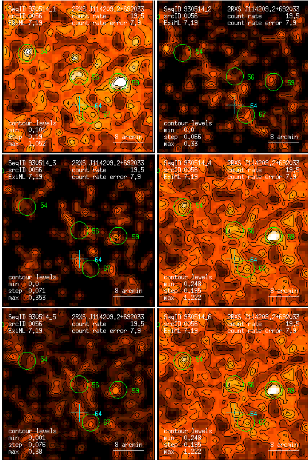
Figure 56: RASS 930514: detection 0056: band rate images, Gaussian filter: (1) PSPC channels 11 – 41, (2) 52 – 90, (3) 91 – 201, (4) 11 – 235, (5) 52 – 201, (6) 11 – 201. Broad band rates in counts/ks. Band rate contour levels in counts/ks/arcmin 2 .
