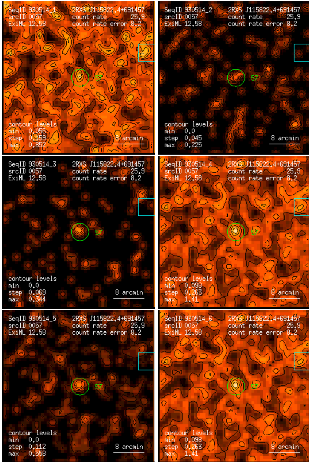
Figure 57: RASS 930514: detection 0057: band rate images, Gaussian filter: (1) PSPC channels 11 – 41, (2) 52 – 90, (3) 91 – 201, (4) 11 – 235, (5) 52 – 201, (6) 11 – 201. Broad band rates in counts/ks. Band rate contour levels in counts/ks/arcmin 2 .
