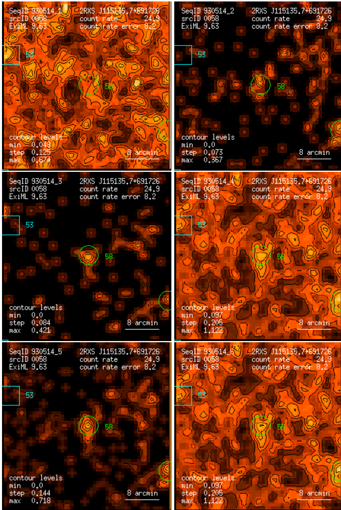
Figure 58: RASS 930514: detection 0058: band rate images, Gaussian filter: (1) PSPC channels 11 – 41, (2) 52 – 90, (3) 91 – 201, (4) 11 – 235, (5) 52 – 201, (6) 11 – 201. Broad band rates in counts/ks. Band rate contour levels in counts/ks/arcmin 2 .
