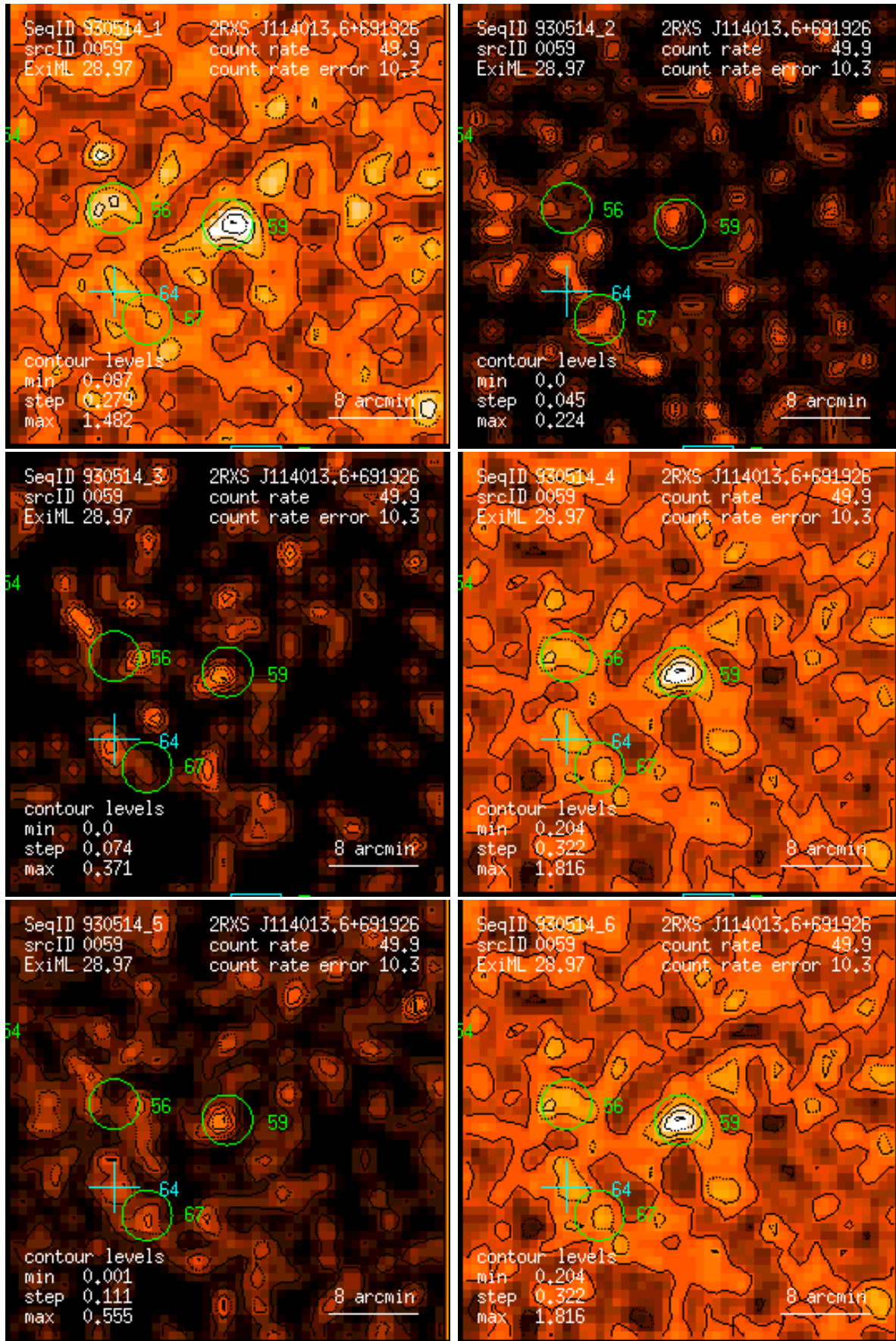
Figure 59: RASS 930514: detection 0059: band rate images, Gaussian filter: (1) PSPC channels 11 – 41, (2) 52 – 90, (3) 91 – 201, (4) 11 – 235, (5) 52 – 201, (6) 11 – 201. Broad band rates in counts/ks. Band rate contour levels in counts/ks/arcmin 2 .
