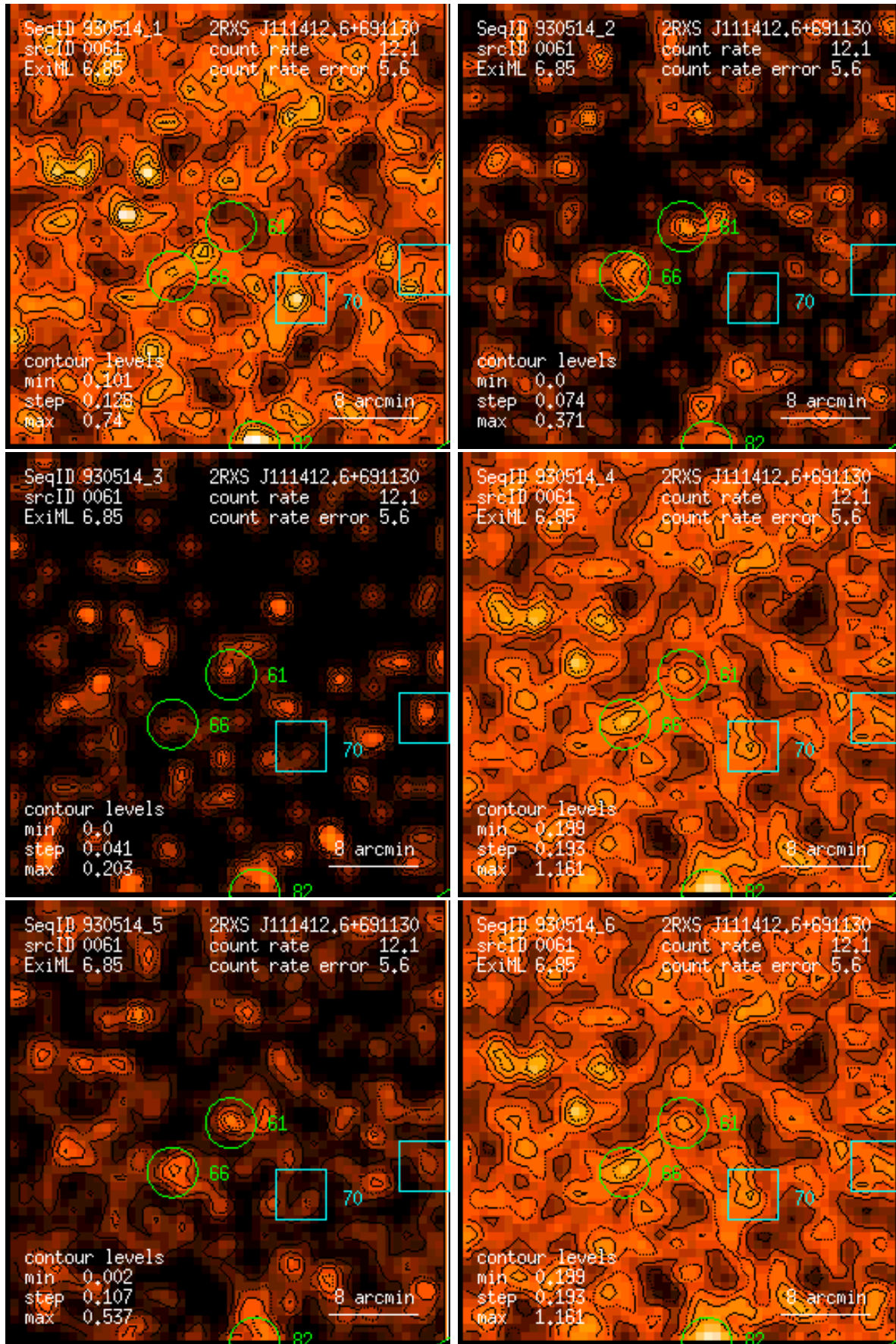
Figure 61: RASS 930514: detection 0061: band rate images, Gaussian filter: (1) PSPC channels 11 – 41, (2) 52 – 90, (3) 91 – 201, (4) 11 – 235, (5) 52 – 201, (6) 11 – 201. Broad band rates in counts/ks. Band rate contour levels in counts/ks/arcmin 2 .
