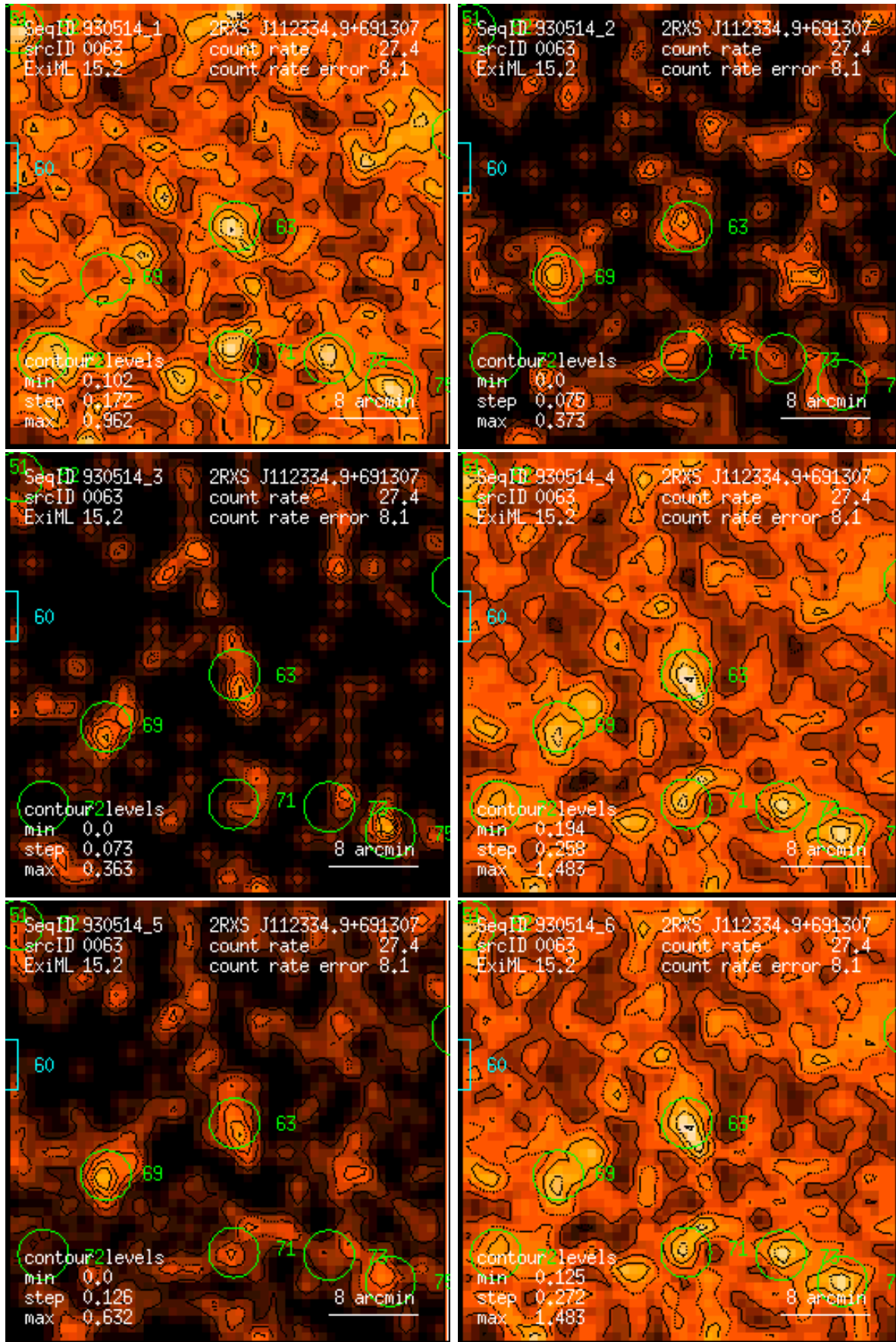
Figure 63: RASS 930514: detection 0063: band rate images, Gaussian filter: (1) PSPC channels 11 – 41, (2) 52 – 90, (3) 91 – 201, (4) 11 – 235, (5) 52 – 201, (6) 11 – 201. Broad band rates in counts/ks. Band rate contour levels in counts/ks/arcmin 2 .
