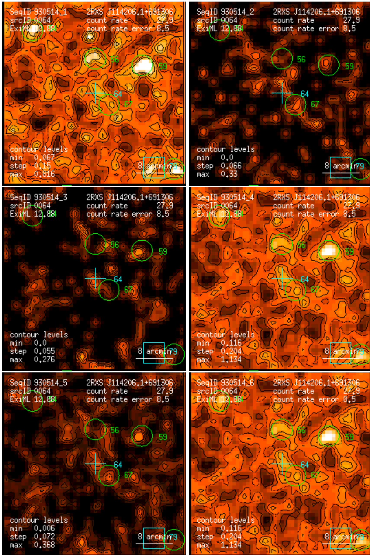
Figure 64: RASS 930514: detection 0064: band rate images, Gaussian filter: (1) PSPC channels 11 – 41, (2) 52 – 90, (3) 91 – 201, (4) 11 – 235, (5) 52 – 201, (6) 11 – 201. Broad band rates in counts/ks. Band rate contour levels in counts/ks/arcmin 2 .
