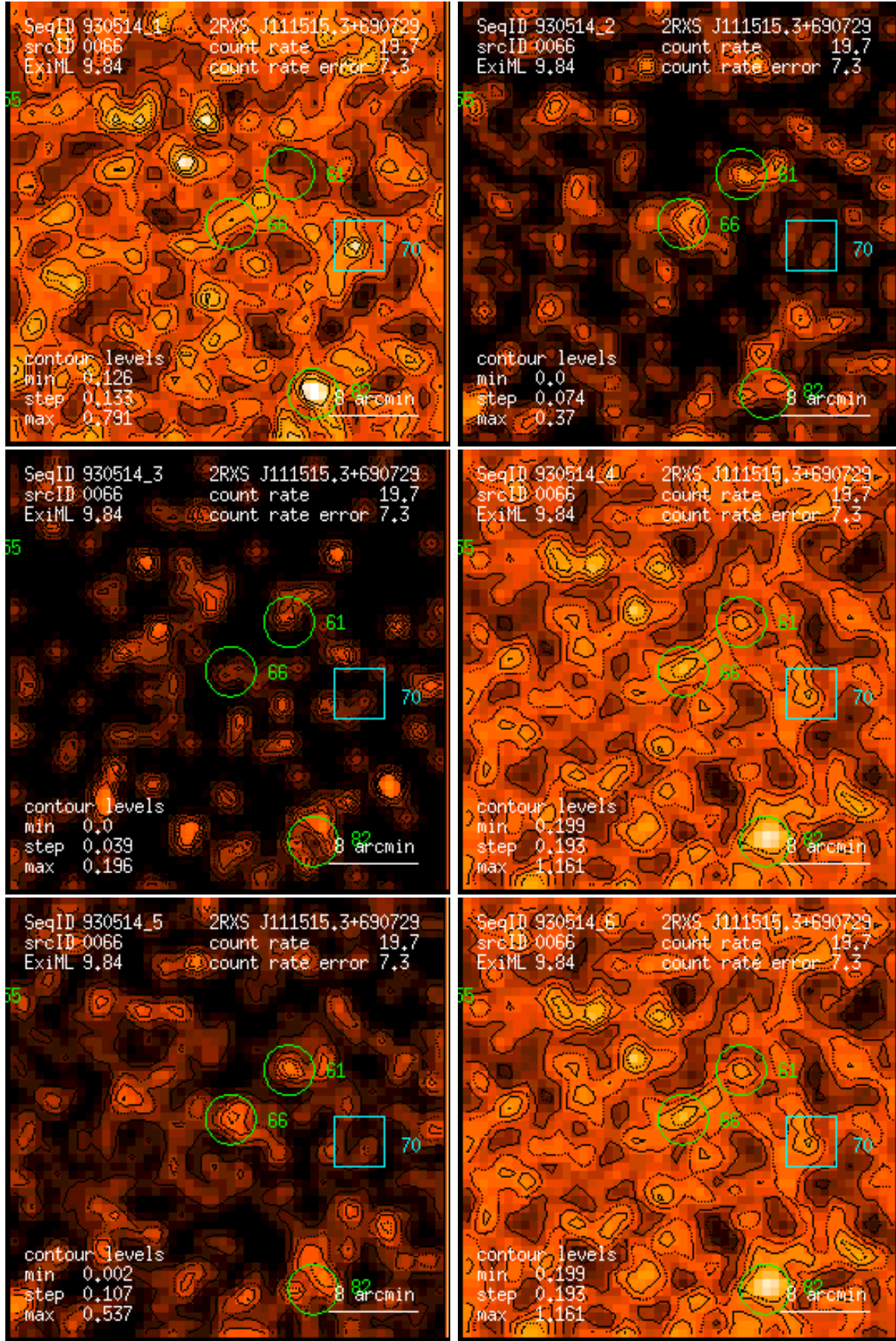
Figure 66: RASS 930514: detection 0066: band rate images, Gaussian filter: (1) PSPC channels 11 – 41, (2) 52 – 90, (3) 91 – 201, (4) 11 – 235, (5) 52 – 201, (6) 11 – 201. Broad band rates in counts/ks. Band rate contour levels in counts/ks/arcmin 2 .
