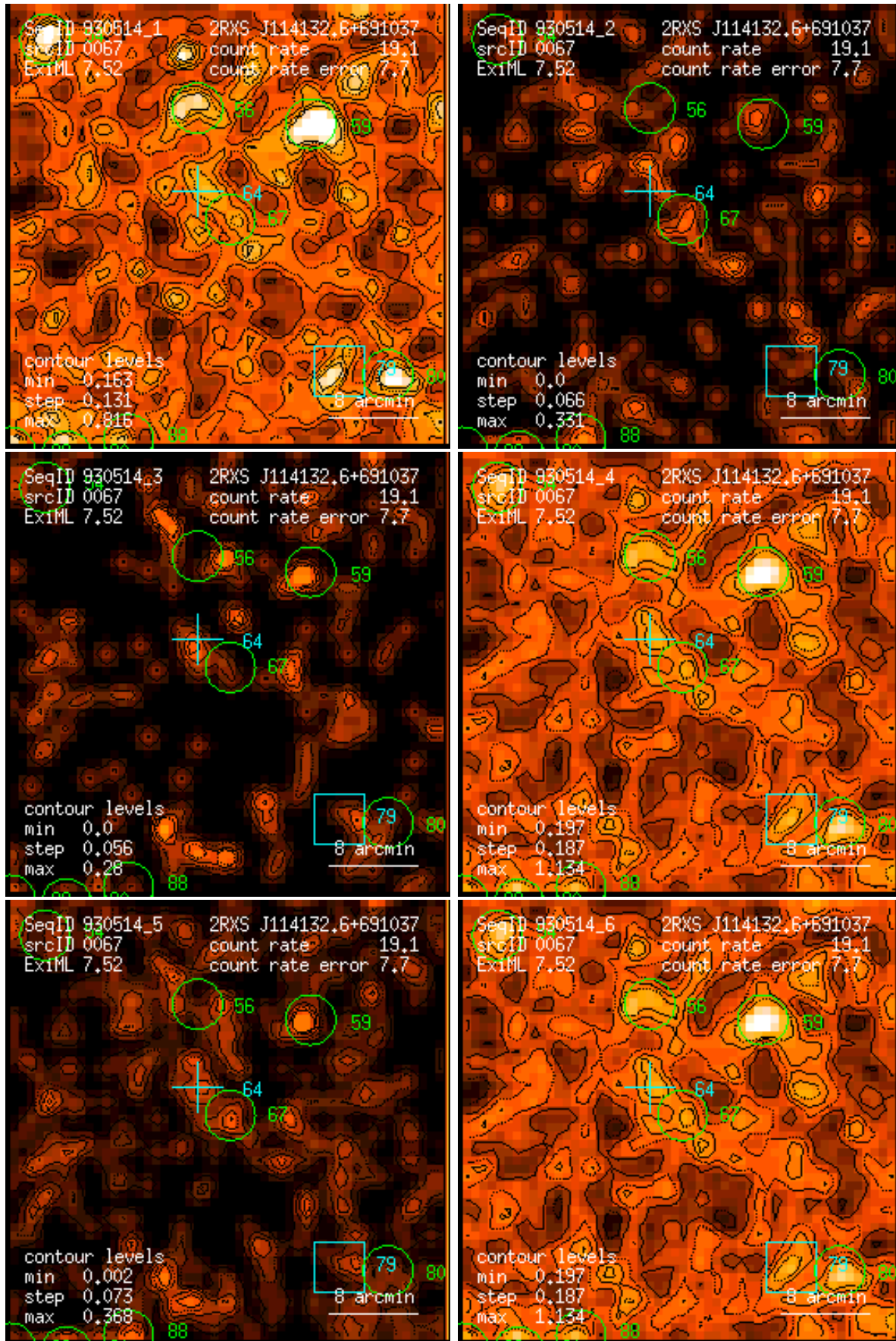
Figure 67: RASS 930514: detection 0067: band rate images, Gaussian filter: (1) PSPC channels 11 – 41, (2) 52 – 90, (3) 91 – 201, (4) 11 – 235, (5) 52 – 201, (6) 11 – 201. Broad band rates in counts/ks. Band rate contour levels in counts/ks/arcmin 2 .
