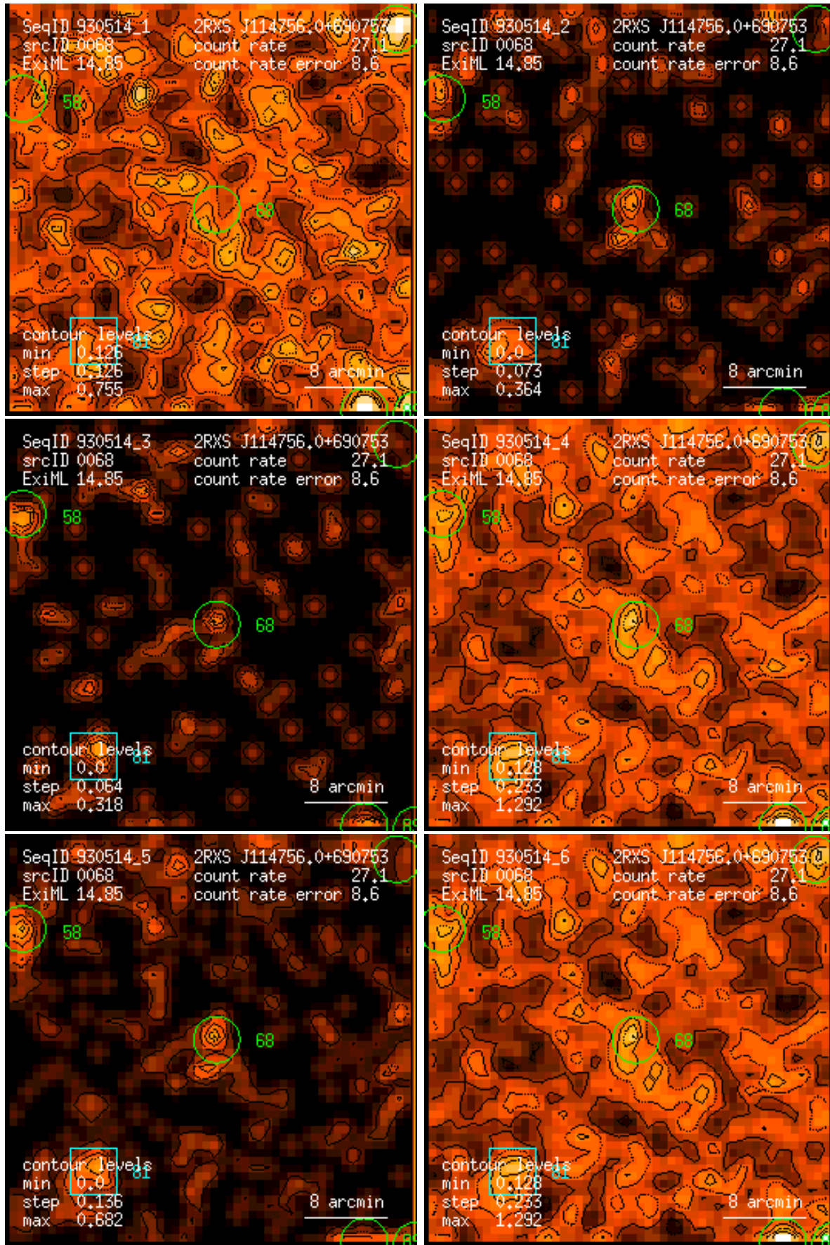
Figure 68: RASS 930514: detection 0068: band rate images, Gaussian filter: (1) PSPC channels 11 – 41, (2) 52 – 90, (3) 91 – 201, (4) 11 – 235, (5) 52 – 201, (6) 11 – 201. Broad band rates in counts/ks. Band rate contour levels in counts/ks/arcmin 2 .
