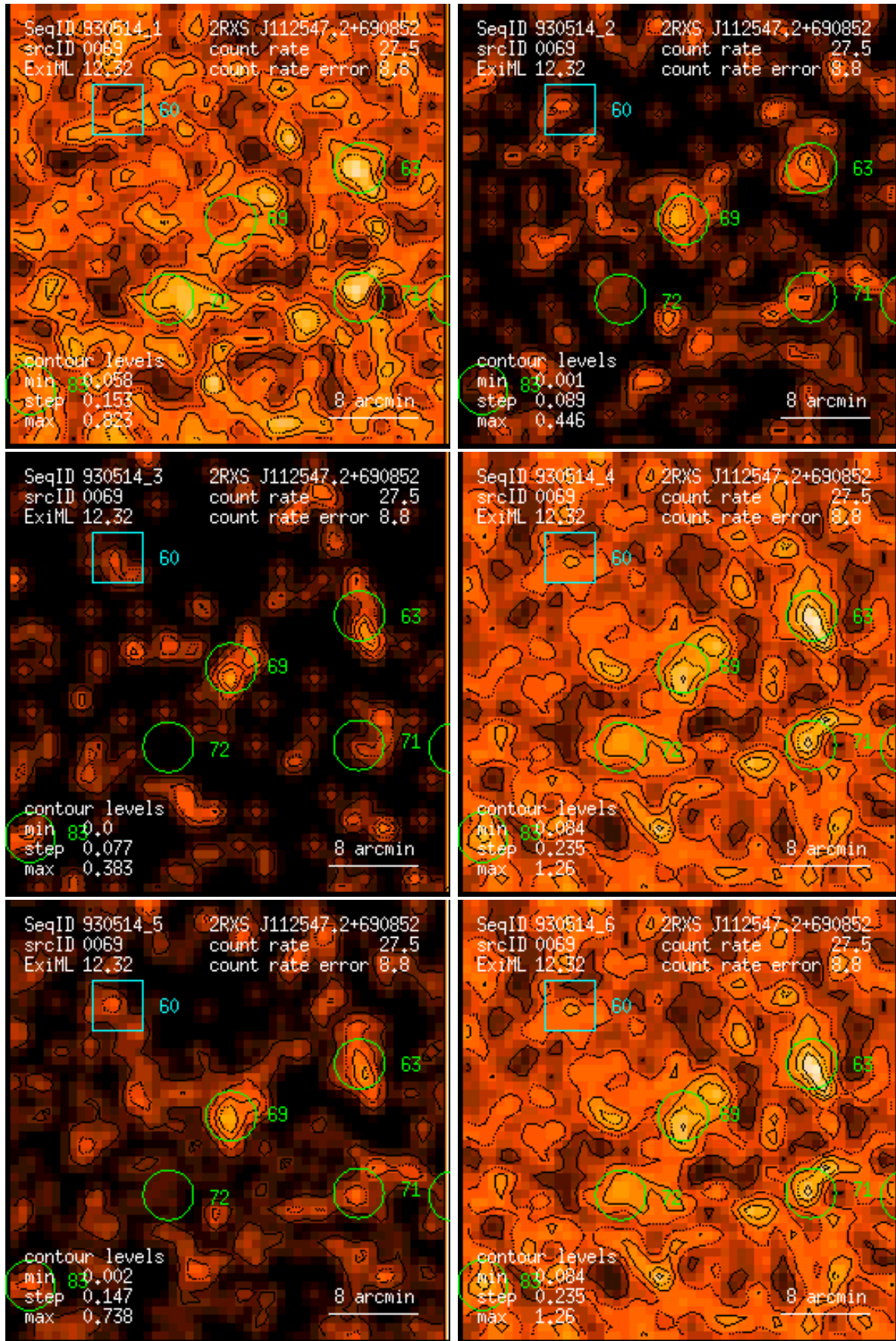
Figure 69: RASS 930514: detection 0069: band rate images, Gaussian filter: (1) PSPC channels 11 – 41, (2) 52 – 90, (3) 91 – 201, (4) 11 – 235, (5) 52 – 201, (6) 11 – 201. Broad band rates in counts/ks. Band rate contour levels in counts/ks/arcmin 2 .
