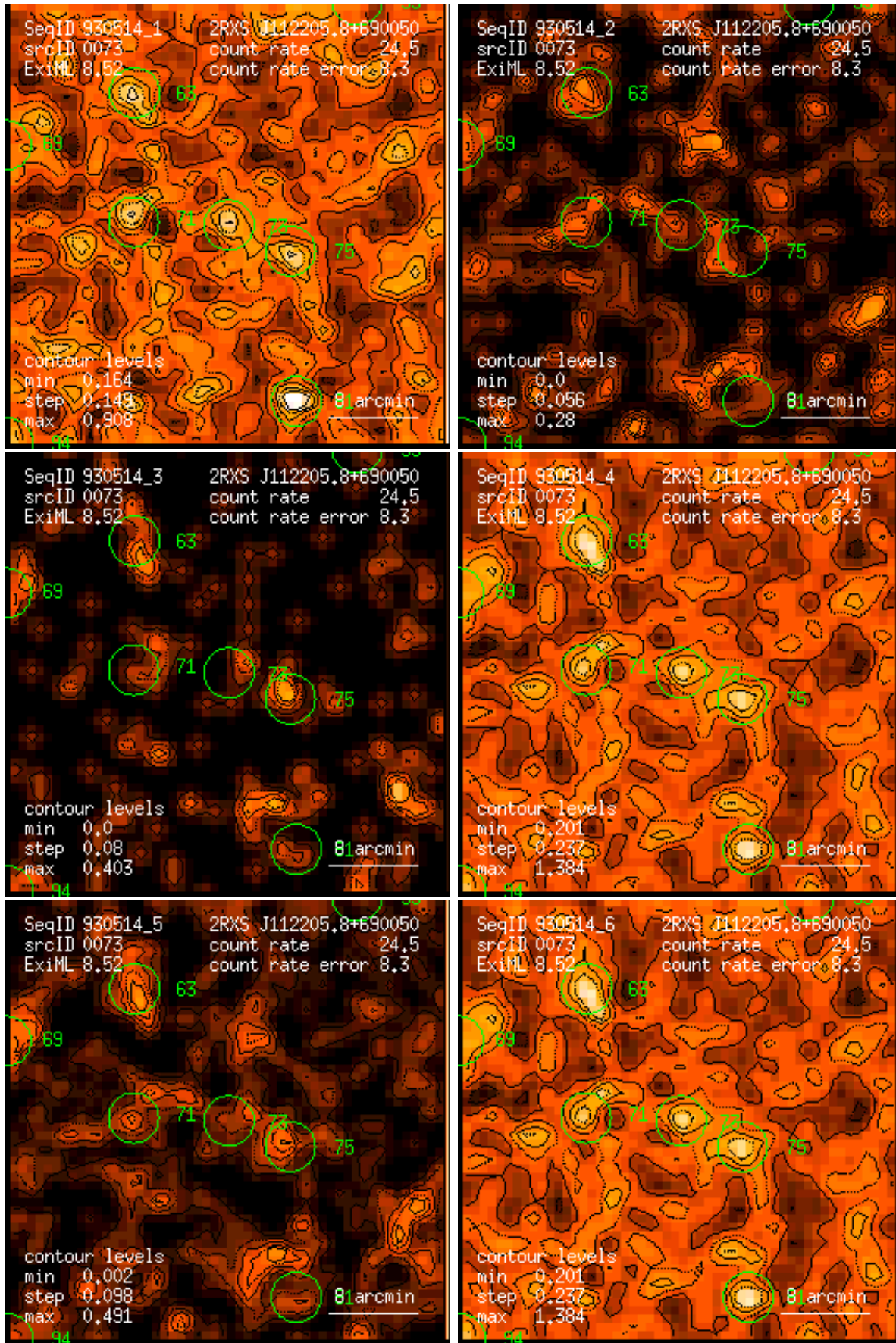
Figure 73: RASS 930514: detection 0073: band rate images, Gaussian filter: (1) PSPC channels 11 – 41, (2) 52 – 90, (3) 91 – 201, (4) 11 – 235, (5) 52 – 201, (6) 11 – 201. Broad band rates in counts/ks. Band rate contour levels in counts/ks/arcmin 2 .
