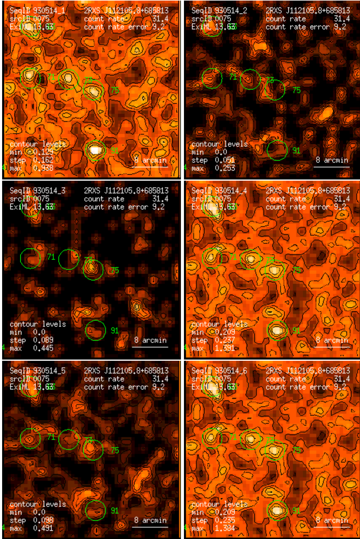
Figure 75: RASS 930514: detection 0075: band rate images, Gaussian filter: (1) PSPC channels 11 – 41, (2) 52 – 90, (3) 91 – 201, (4) 11 – 235, (5) 52 – 201, (6) 11 – 201. Broad band rates in counts/ks. Band rate contour levels in counts/ks/arcmin 2 .
