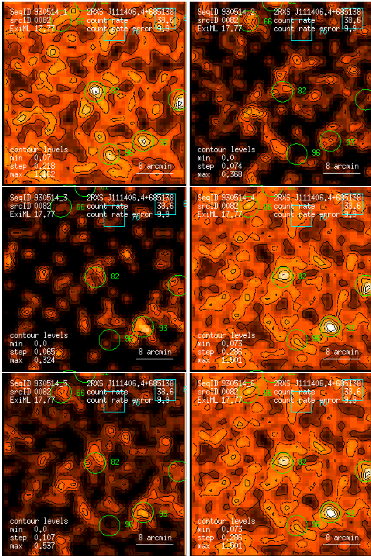
Figure 82: RASS 930514: detection 0082: band rate images, Gaussian filter: (1) PSPC channels 11 – 41, (2) 52 – 90, (3) 91 – 201, (4) 11 – 235, (5) 52 – 201, (6) 11 – 201. Broad band rates in counts/ks. Band rate contour levels in counts/ks/arcmin 2 .
