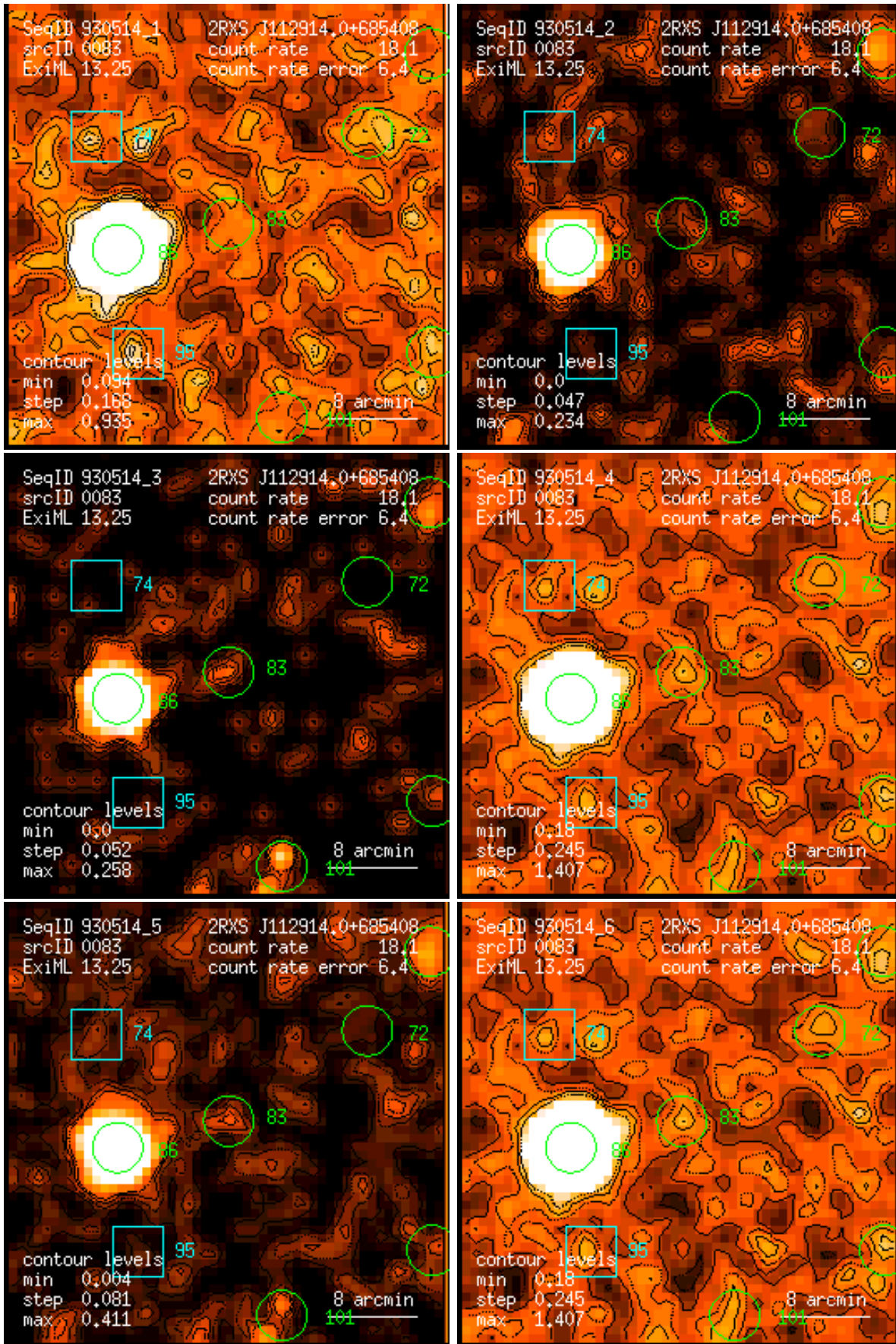
Figure 83: RASS 930514: detection 0083: band rate images, Gaussian filter: (1) PSPC channels 11 – 41, (2) 52 – 90, (3) 91 – 201, (4) 11 – 235, (5) 52 – 201, (6) 11 – 201. Broad band rates in counts/ks. Band rate contour levels in counts/ks/arcmin 2 .
