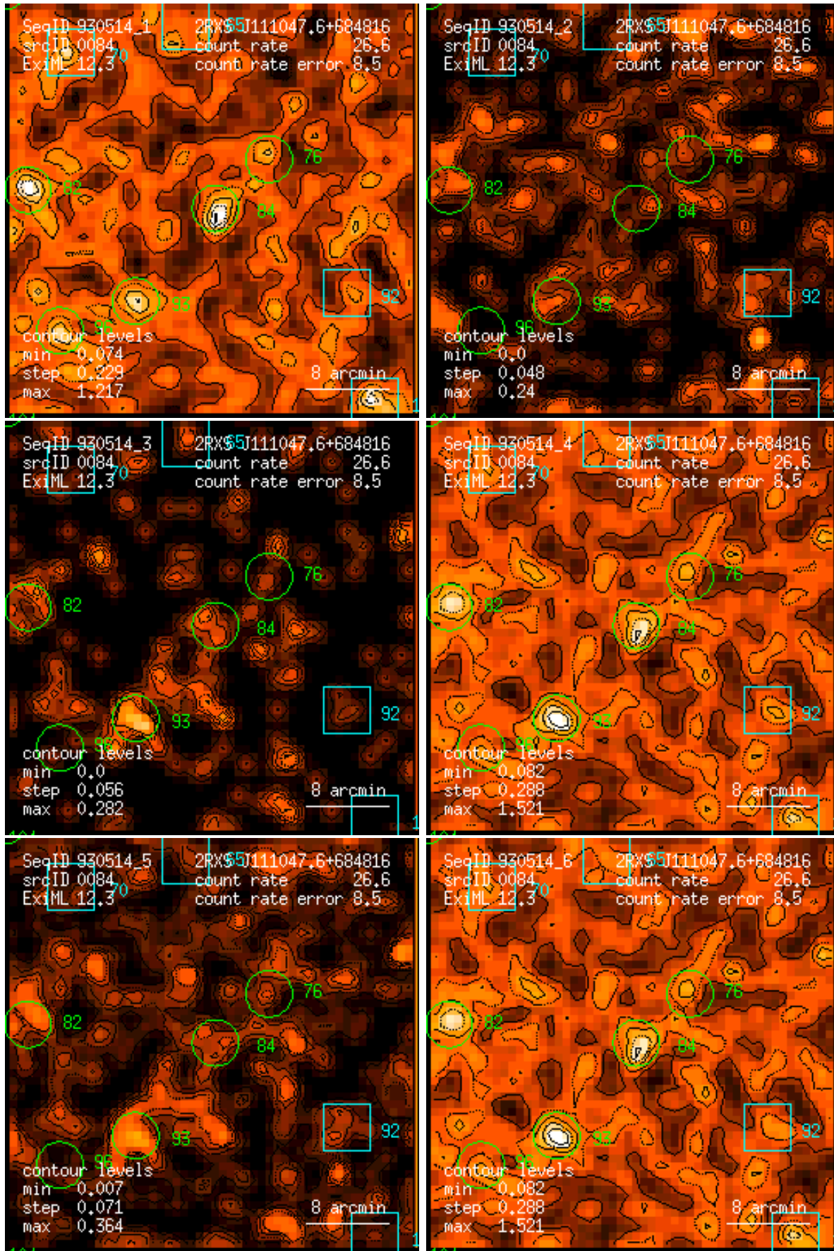
Figure 84: RASS 930514: detection 0084: band rate images, Gaussian filter: (1) PSPC channels 11 – 41, (2) 52 – 90, (3) 91 – 201, (4) 11 – 235, (5) 52 – 201, (6) 11 – 201. Broad band rates in counts/ks. Band rate contour levels in counts/ks/arcmin 2 .
