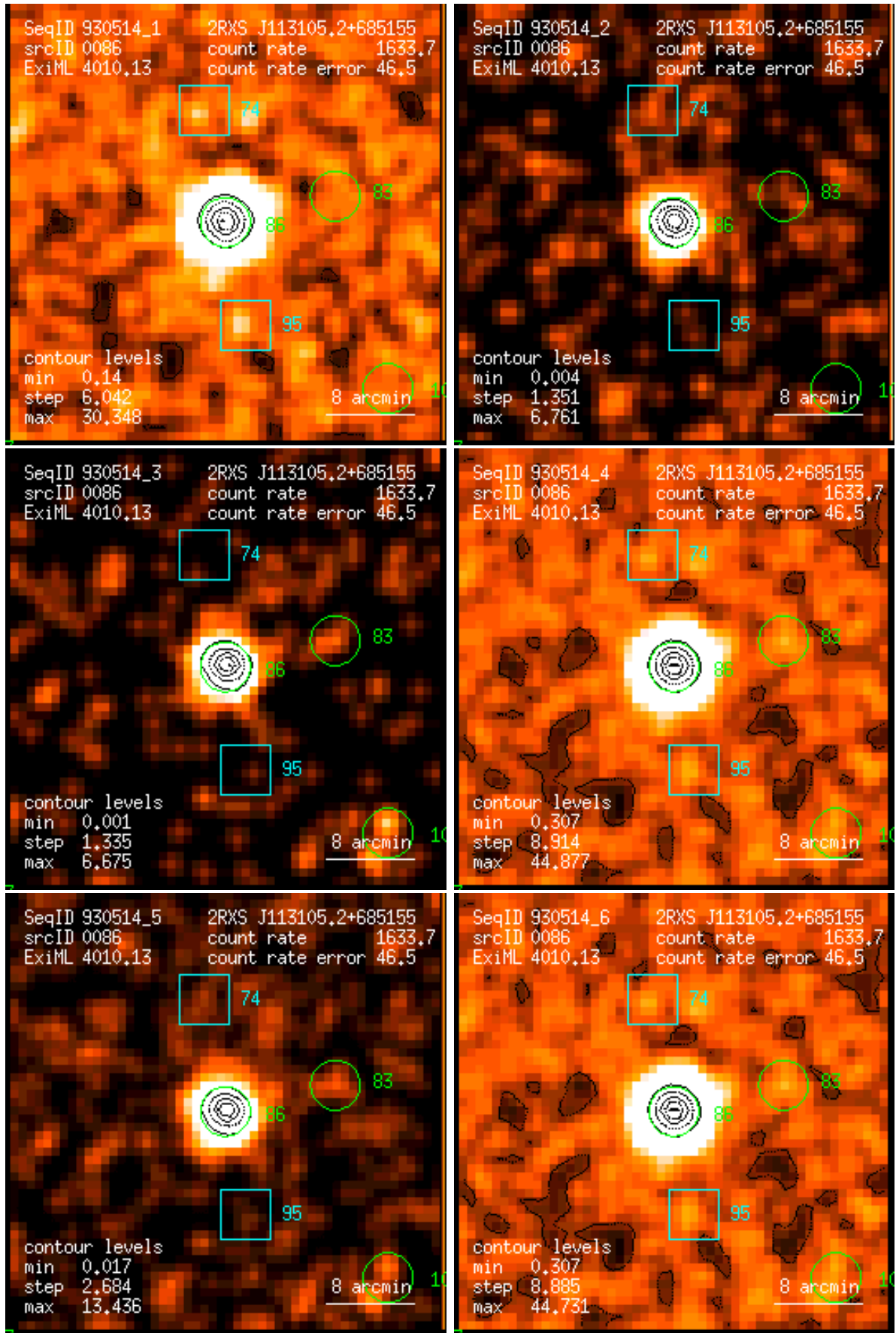
Figure 86: RASS 930514: detection 0086: band rate images, Gaussian filter: (1) PSPC channels 11 – 41, (2) 52 – 90, (3) 91 – 201, (4) 11 – 235, (5) 52 – 201, (6) 11 – 201. Broad band rates in counts/ks. Band rate contour levels in counts/ks/arcmin 2 .
