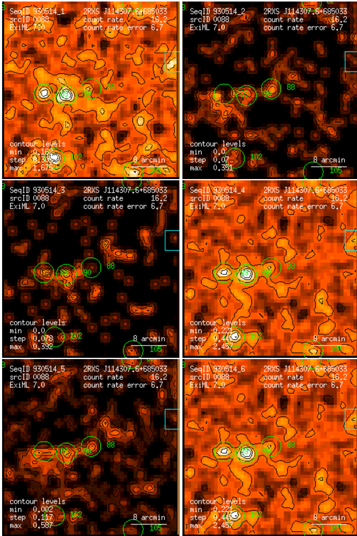
Figure 88: RASS 930514: detection 0088: band rate images, Gaussian filter: (1) PSPC channels 11 – 41, (2) 52 – 90, (3) 91 – 201, (4) 11 – 235, (5) 52 – 201, (6) 11 – 201. Broad band rates in counts/ks. Band rate contour levels in counts/ks/arcmin 2 .
