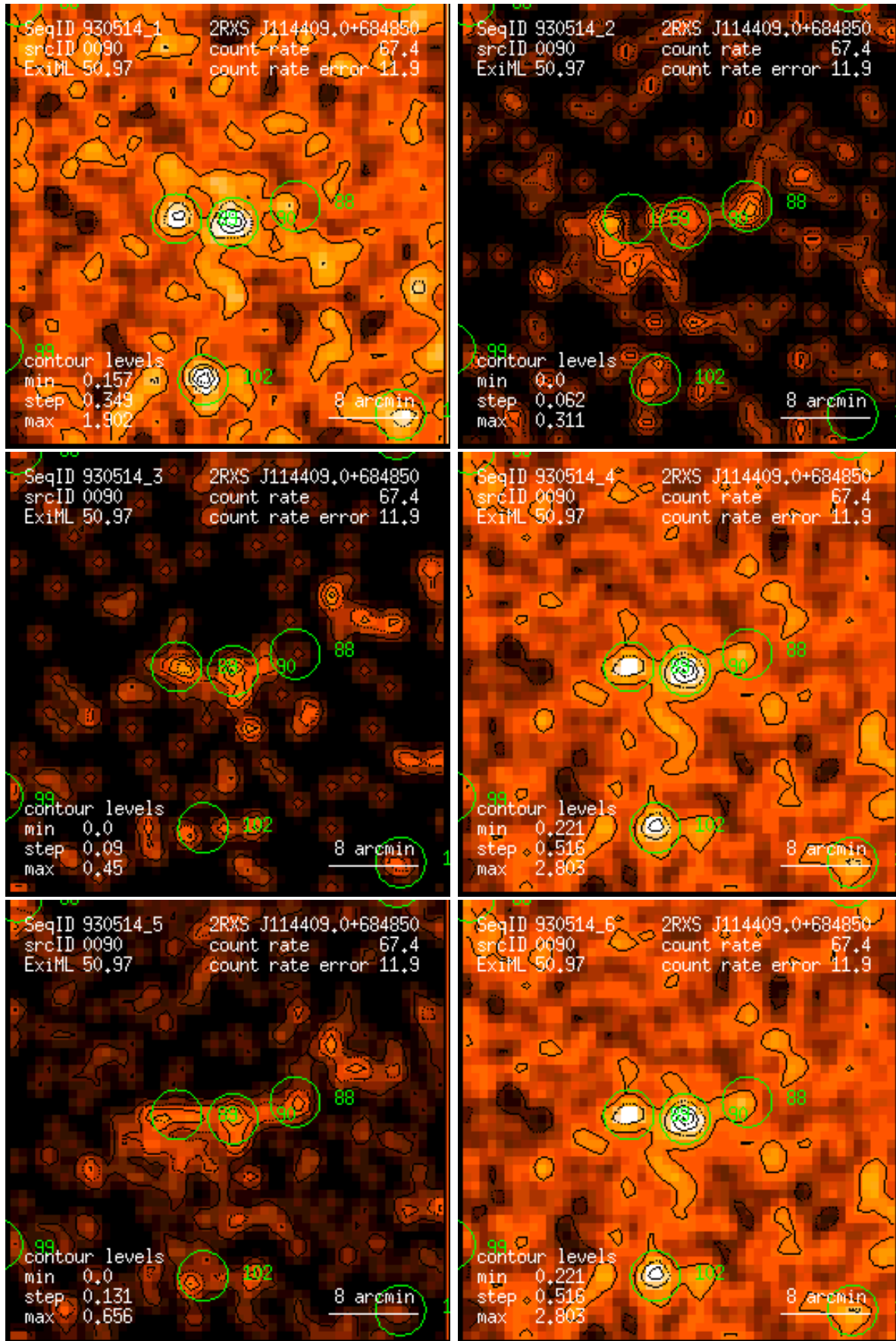
Figure 90: RASS 930514: detection 0090: band rate images, Gaussian filter: (1) PSPC channels 11 – 41, (2) 52 – 90, (3) 91 – 201, (4) 11 – 235, (5) 52 – 201, (6) 11 – 201. Broad band rates in counts/ks. Band rate contour levels in counts/ks/arcmin 2 .
