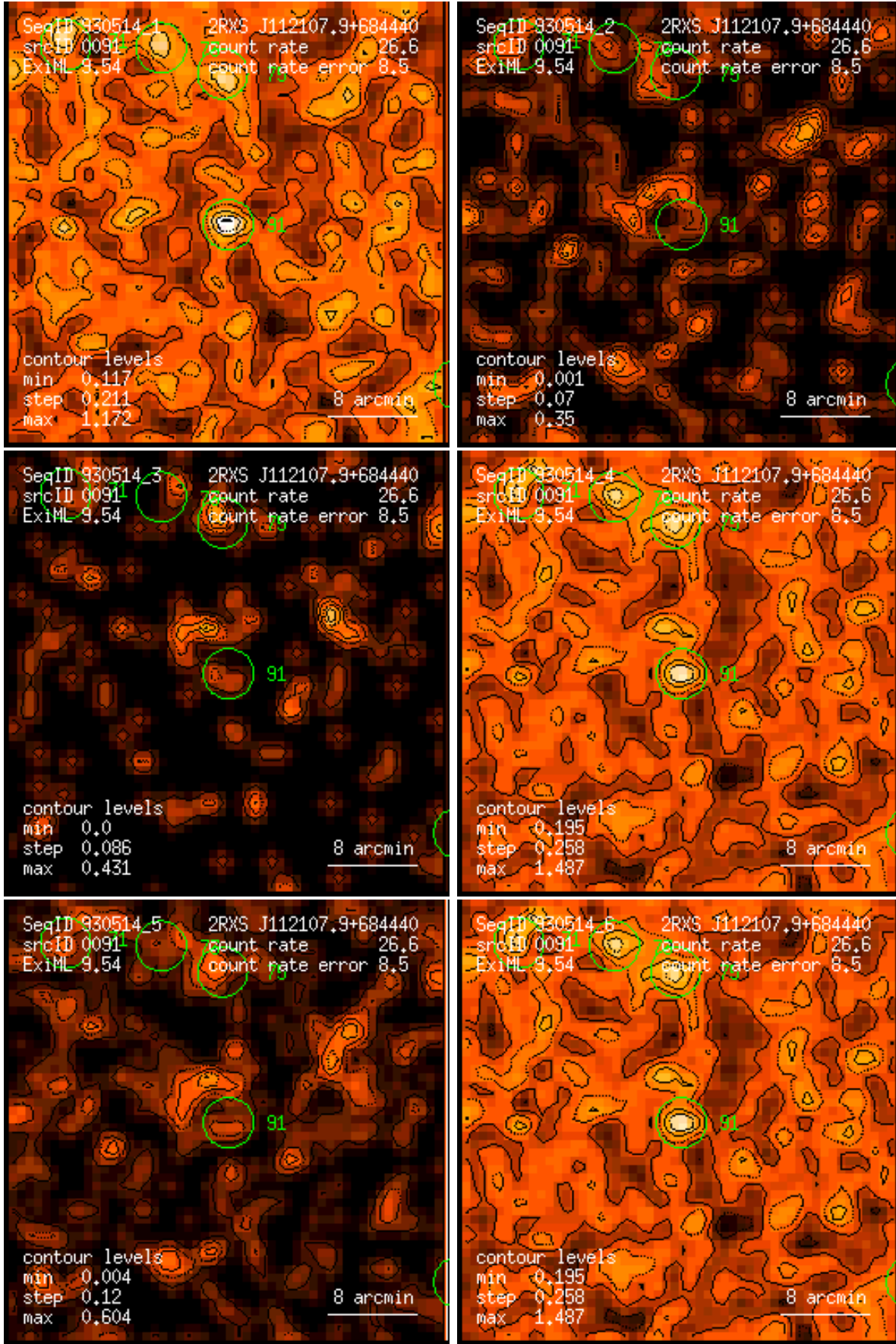
Figure 91: RASS 930514: detection 0091: band rate images, Gaussian filter: (1) PSPC channels 11 – 41, (2) 52 – 90, (3) 91 – 201, (4) 11 – 235, (5) 52 – 201, (6) 11 – 201. Broad band rates in counts/ks. Band rate contour levels in counts/ks/arcmin 2 .
