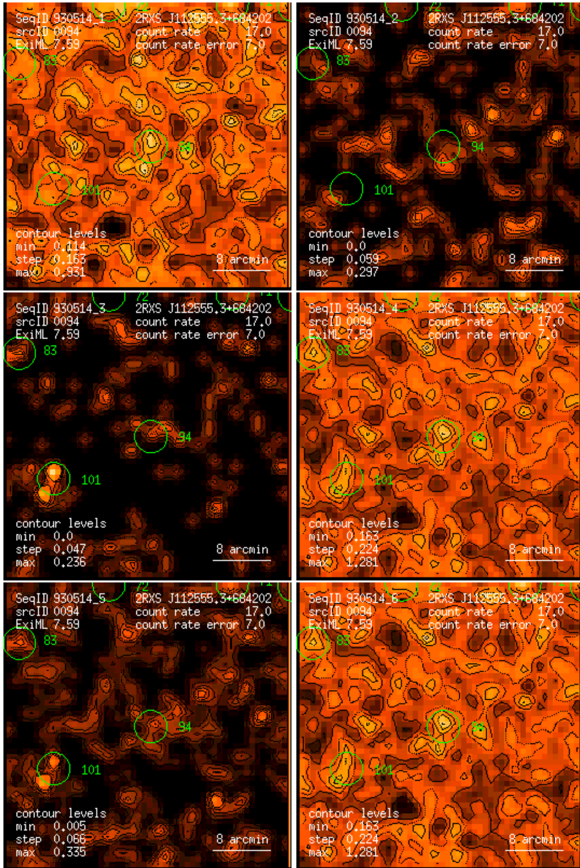
Figure 94: RASS 930514: detection 0094: band rate images, Gaussian filter: (1) PSPC channels 11 – 41, (2) 52 – 90, (3) 91 – 201, (4) 11 – 235, (5) 52 – 201, (6) 11 – 201. Broad band rates in counts/ks. Band rate contour levels in counts/ks/arcmin 2 .
