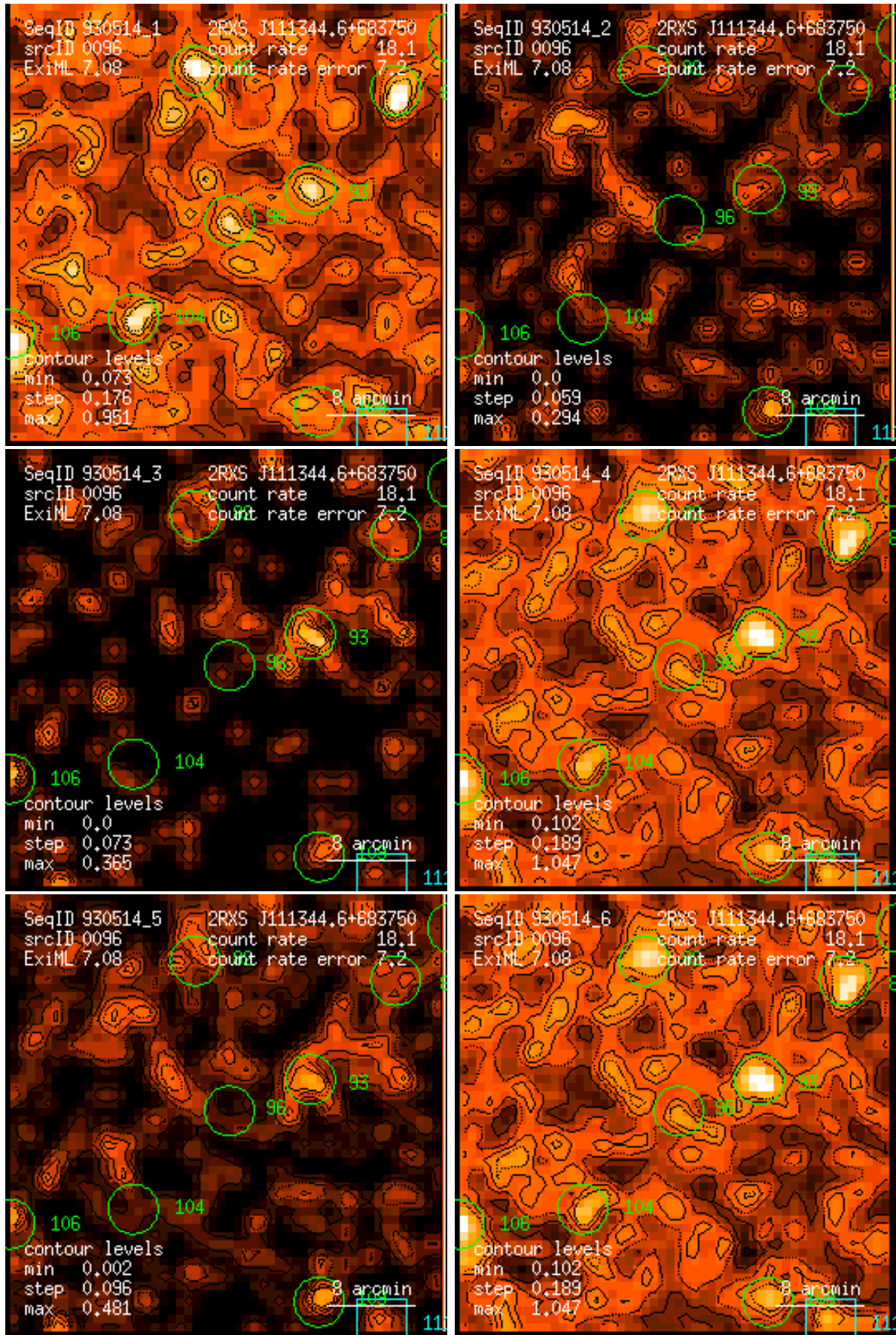
Figure 96: RASS 930514: detection 0096: band rate images, Gaussian filter: (1) PSPC channels 11 – 41, (2) 52 – 90, (3) 91 – 201, (4) 11 – 235, (5) 52 – 201, (6) 11 – 201. Broad band rates in counts/ks. Band rate contour levels in counts/ks/arcmin 2 .
