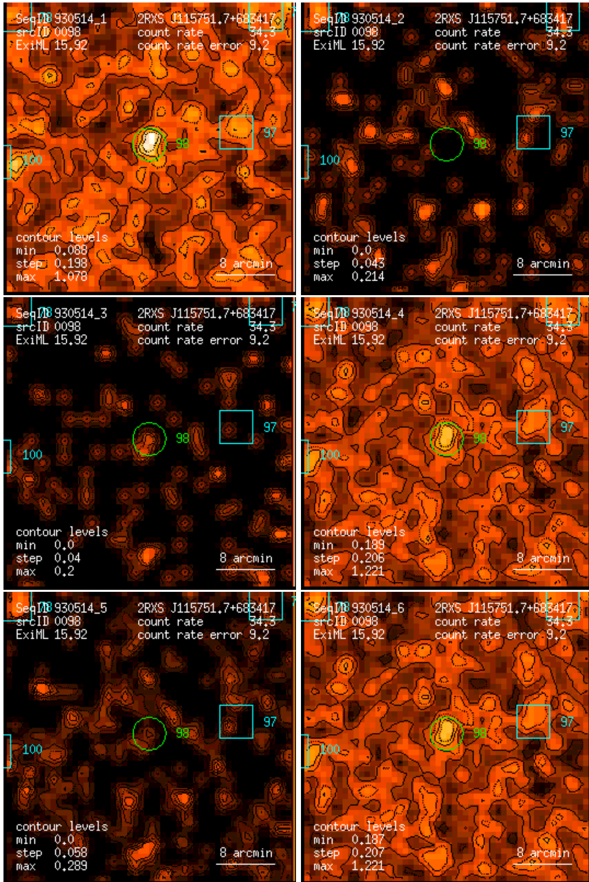
Figure 98: RASS 930514: detection 0098: band rate images, Gaussian filter: (1) PSPC channels 11 – 41, (2) 52 – 90, (3) 91 – 201, (4) 11 – 235, (5) 52 – 201, (6) 11 – 201. Broad band rates in counts/ks. Band rate contour levels in counts/ks/arcmin 2 .
