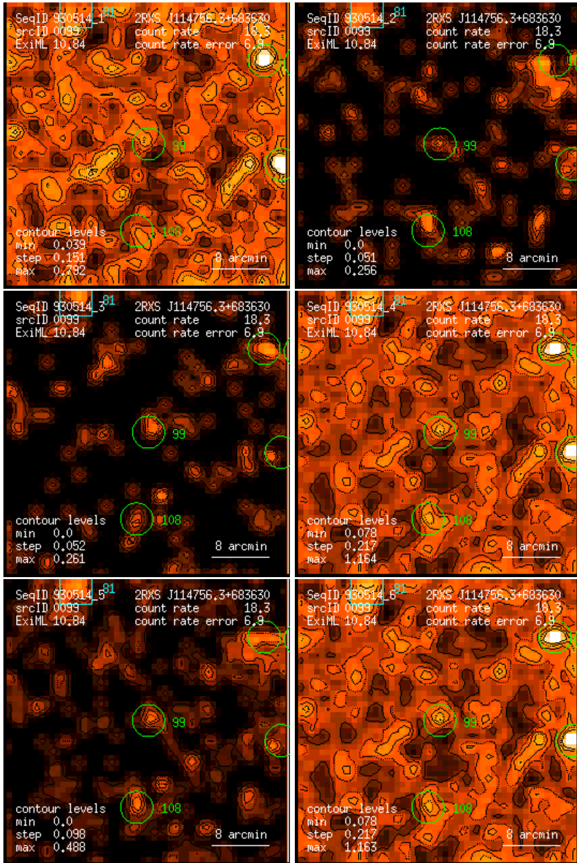
Figure 99: RASS 930514: detection 0099: band rate images, Gaussian filter: (1) PSPC channels 11 – 41, (2) 52 – 90, (3) 91 – 201, (4) 11 – 235, (5) 52 – 201, (6) 11 – 201. Broad band rates in counts/ks. Band rate contour levels in counts/ks/arcmin 2 .
