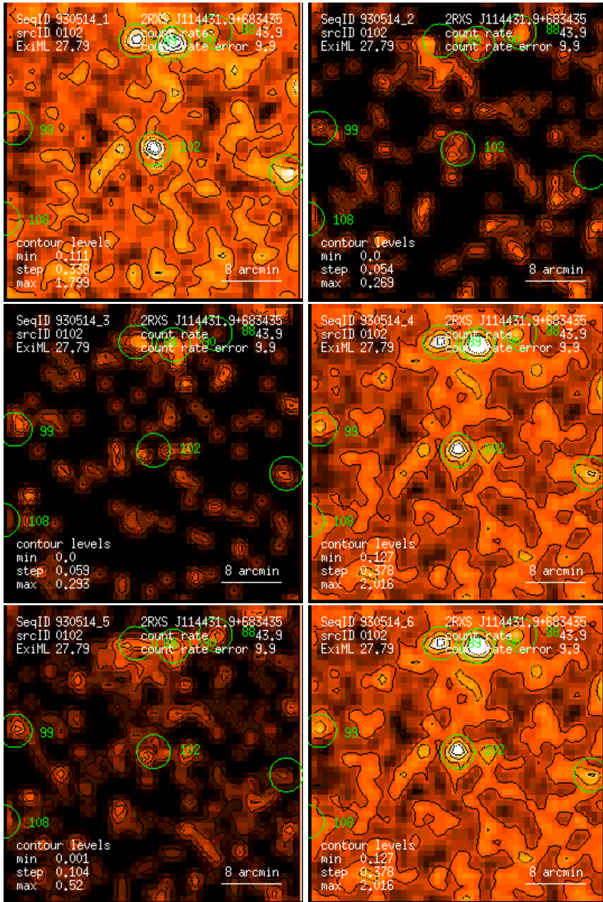
Figure 102: RASS 930514: detection 0102: band rate images, Gaussian filter: (1) PSPC channels 11 – 41, (2) 52 – 90, (3) 91 – 201, (4) 11 – 235, (5) 52 – 201, (6) 11 – 201. Broad band rates in counts/ks. Band rate contour levels in counts/ks/arcmin 2 .
