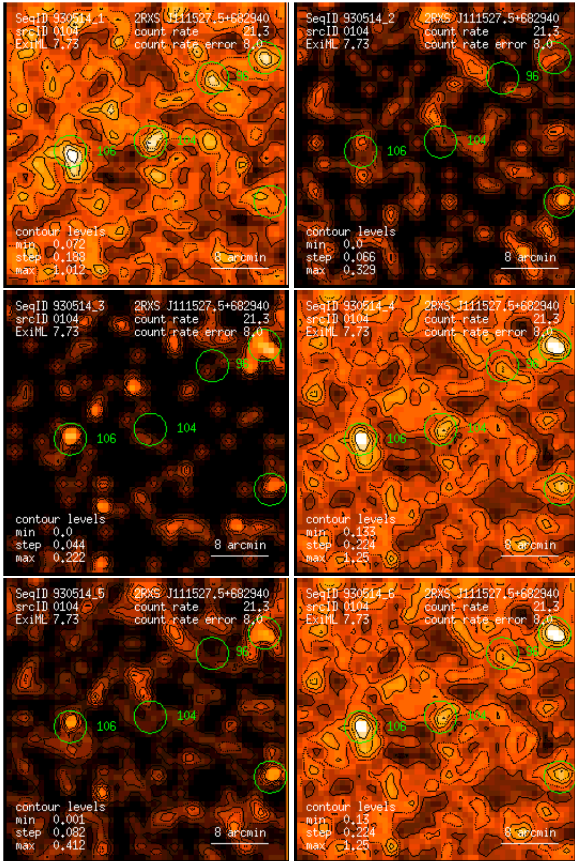
Figure 104: RASS 930514: detection 0104: band rate images, Gaussian filter: (1) PSPC channels 11 – 41, (2) 52 – 90, (3) 91 – 201, (4) 11 – 235, (5) 52 – 201, (6) 11 – 201. Broad band rates in counts/ks. Band rate contour levels in counts/ks/arcmin 2 .
