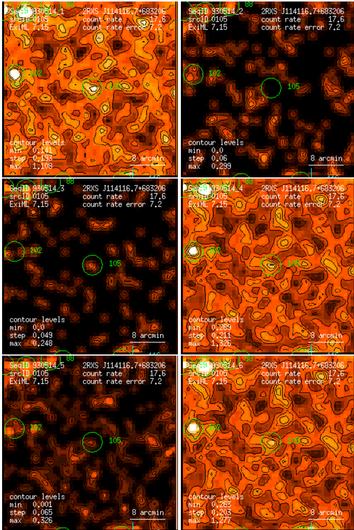
Figure 105: RASS 930514: detection 0105: band rate images, Gaussian filter: (1) PSPC channels 11 – 41, (2) 52 – 90, (3) 91 – 201, (4) 11 – 235, (5) 52 – 201, (6) 11 – 201. Broad band rates in counts/ks. Band rate contour levels in counts/ks/arcmin 2 .
