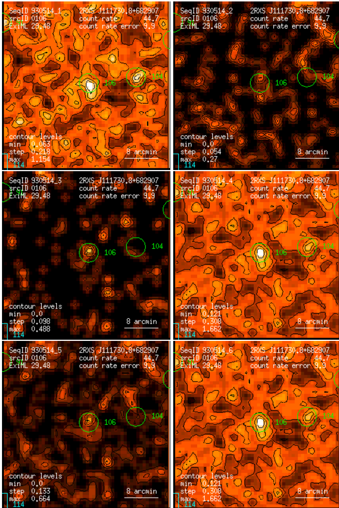
Figure 106: RASS 930514: detection 0106: band rate images, Gaussian filter: (1) PSPC channels 11 – 41, (2) 52 – 90, (3) 91 – 201, (4) 11 – 235, (5) 52 – 201, (6) 11 – 201. Broad band rates in counts/ks. Band rate contour levels in counts/ks/arcmin 2 .
