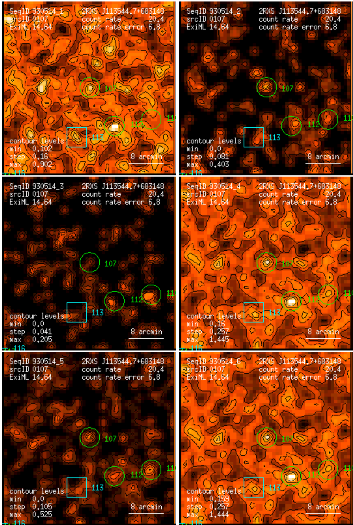
Figure 107: RASS 930514: detection 0107: band rate images, Gaussian filter: (1) PSPC channels 11 – 41, (2) 52 – 90, (3) 91 – 201, (4) 11 – 235, (5) 52 – 201, (6) 11 – 201. Broad band rates in counts/ks. Band rate contour levels in counts/ks/arcmin 2 .
